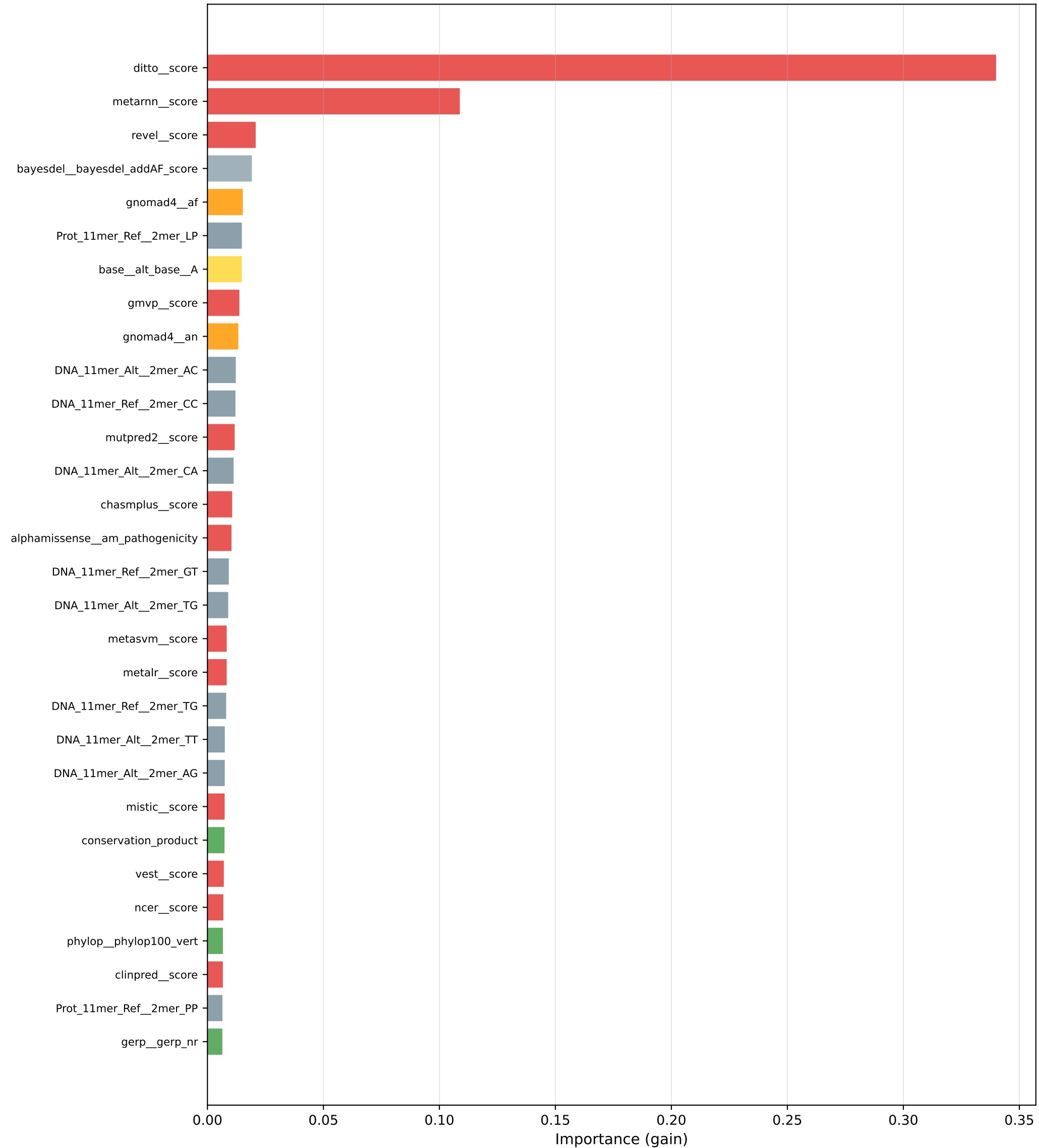
XGBoost
