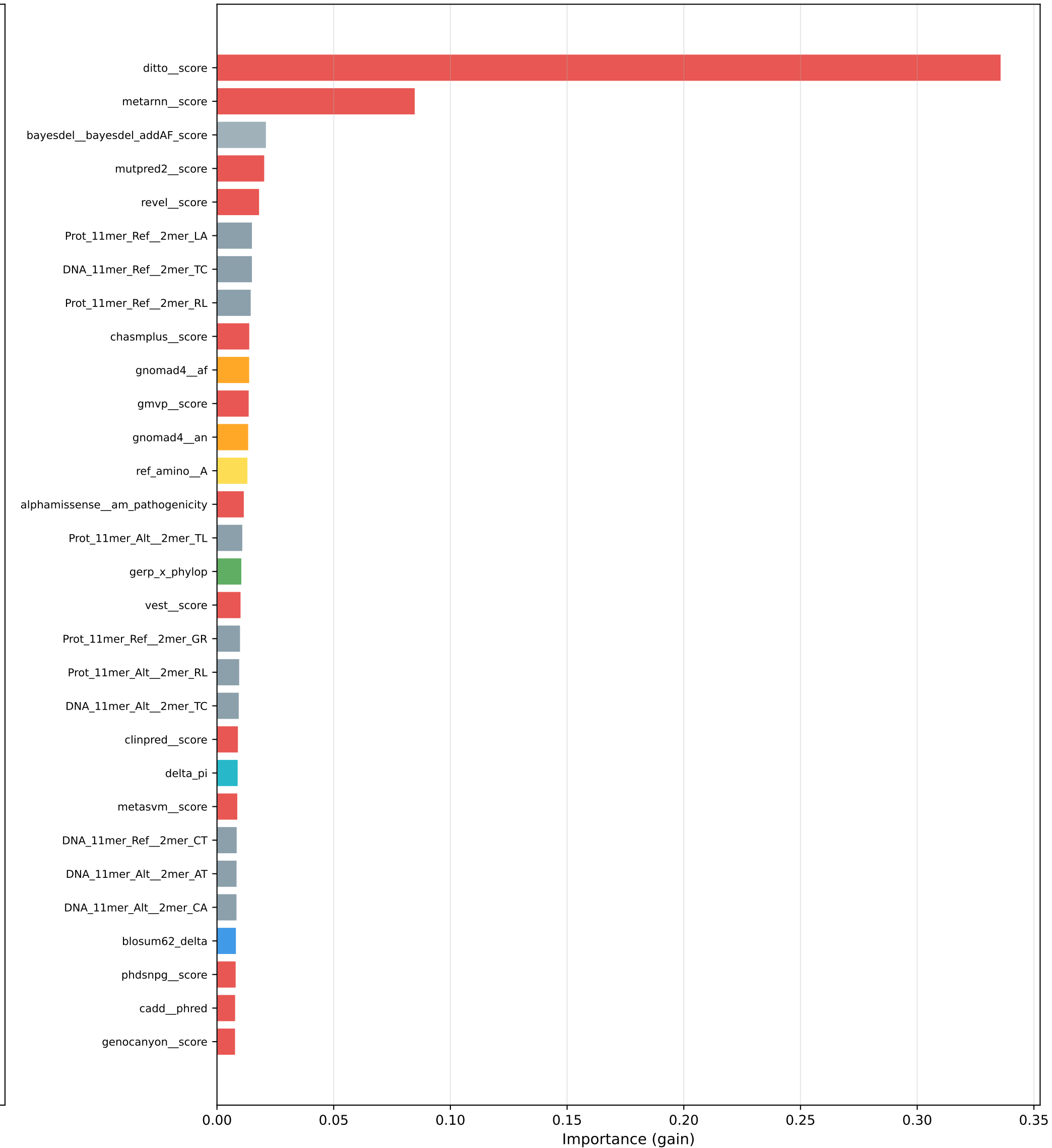
XGBoost
