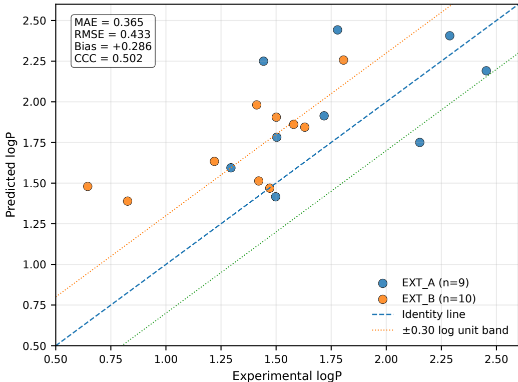
Figure 4 — External validation: Hybrid-XGBoost (EXT-A + EXT-B, n=19)
