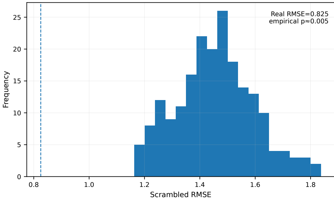
Figure 06 — Y-scrambling (Hybrid-XGB (ECFP2048 r=2 + PhysChem))
