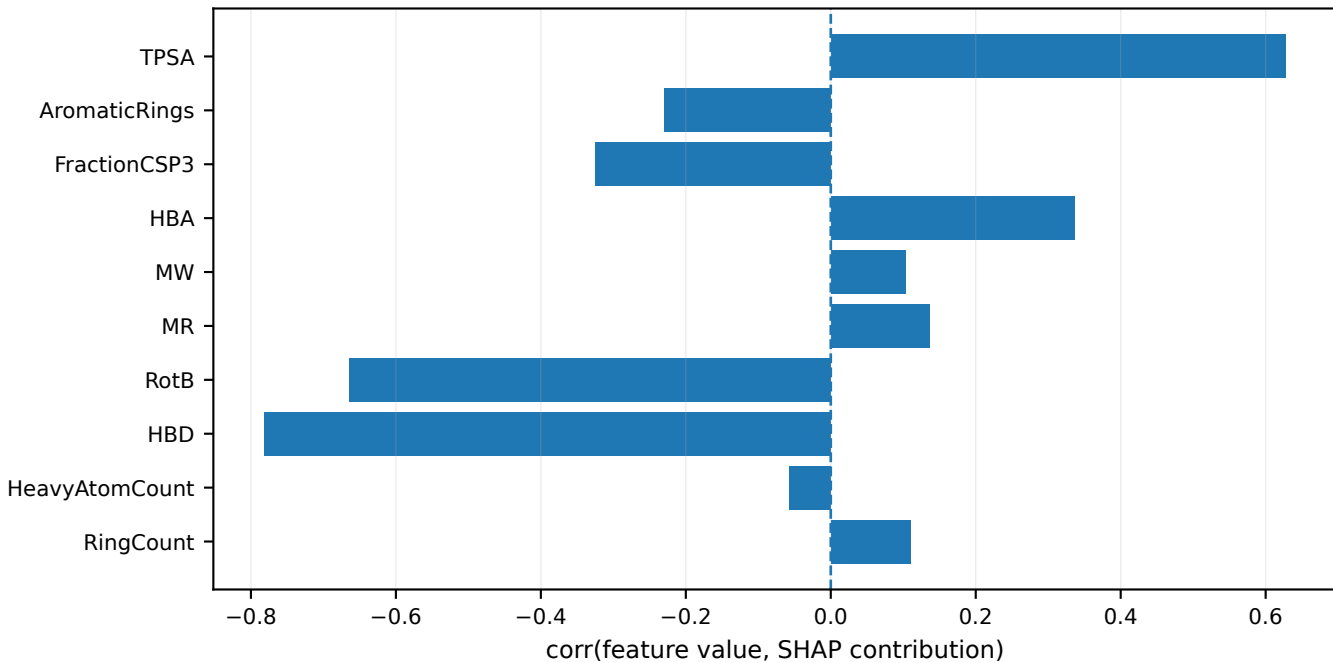
Figure 08 — Directionality (corr(feature, SHAP))
