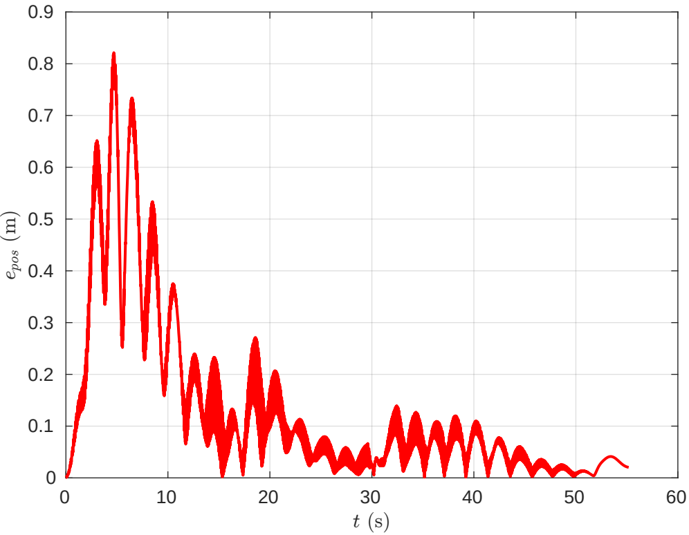
Drone 3 - 3D Position Error vs Time
