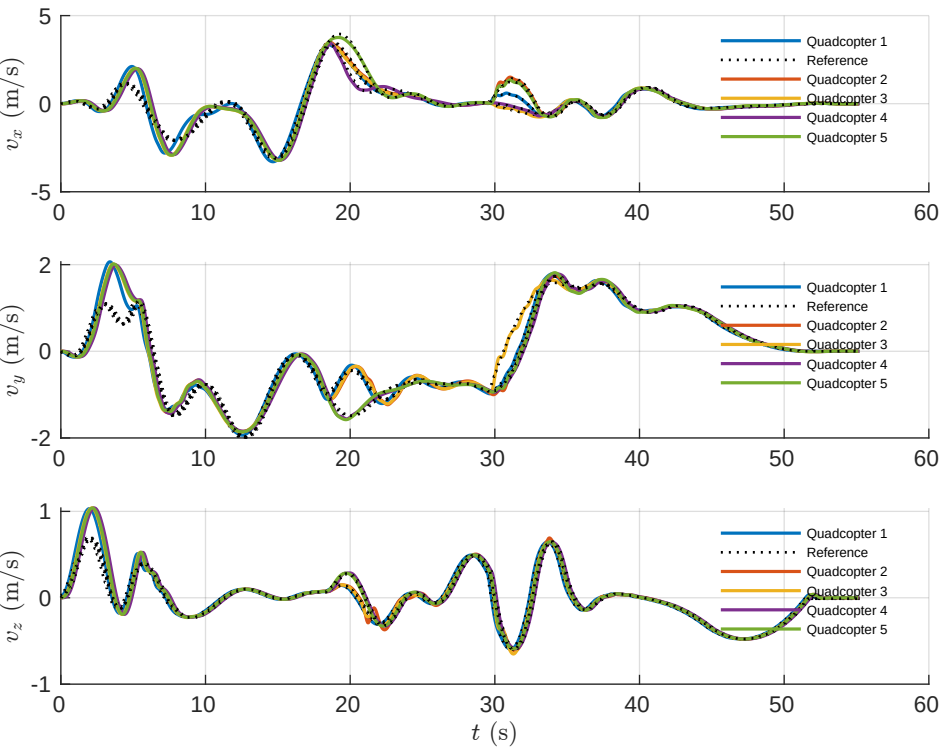
All Drones - Velocity (Actual vs Reference) vs Time
