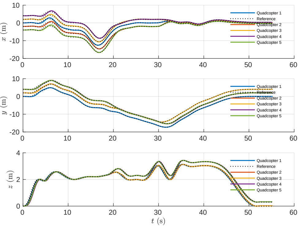
All Drones - Position (Actual vs Reference) vs Time
