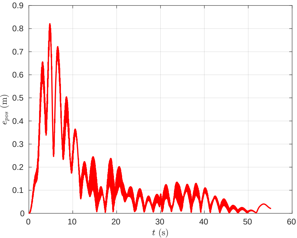
Drone 2 - 3D Position Error vs Time
