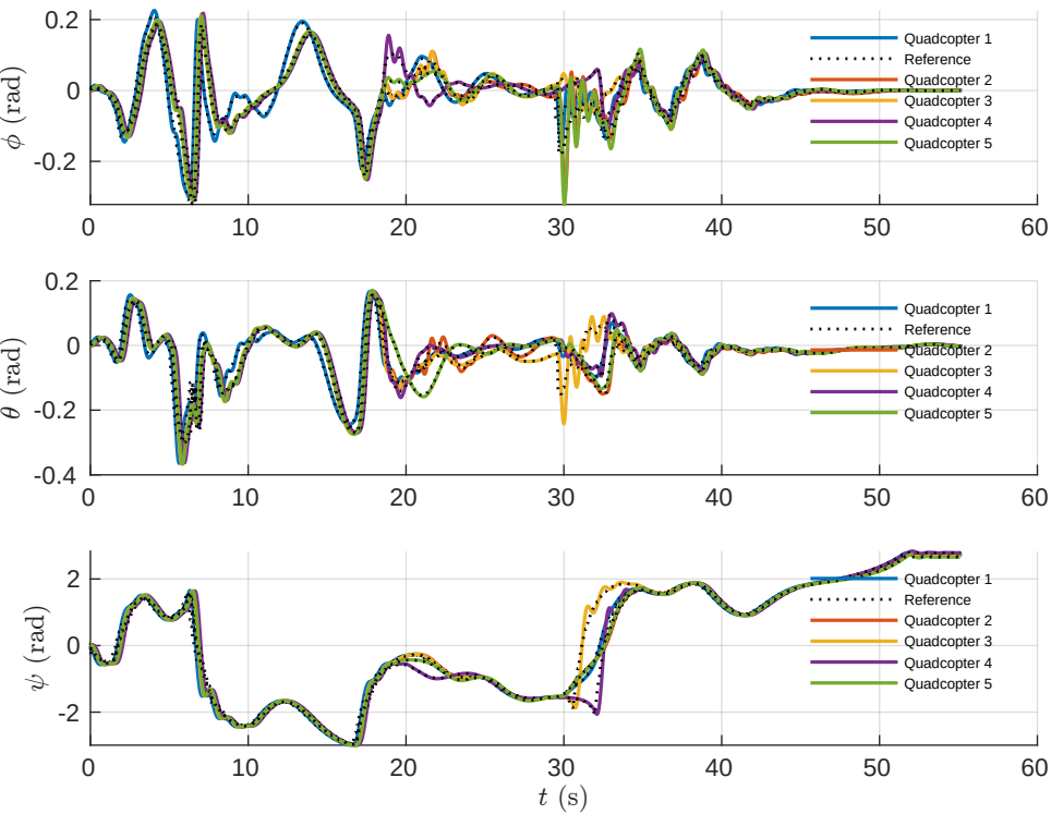
All Drones - Euler Angles (Actual vs Reference) vs Time
