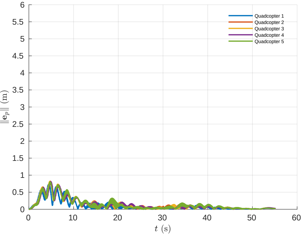
All Drones - 3D Position Error vs Time
