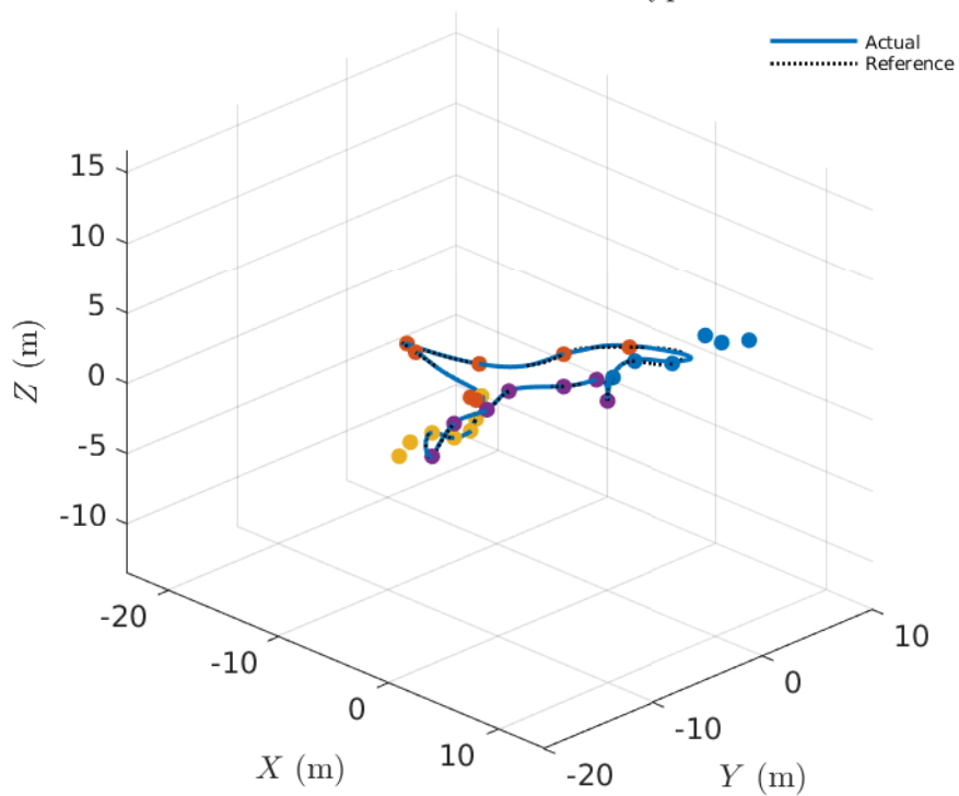
Drone 1 - 3D Position + Waypoints
