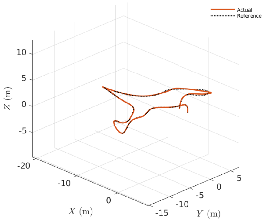
Drone 2 - 3D Position + Waypoints
