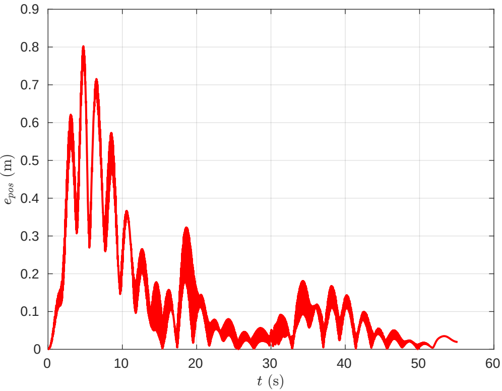
Drone 5 - 3D Position Error vs Time
