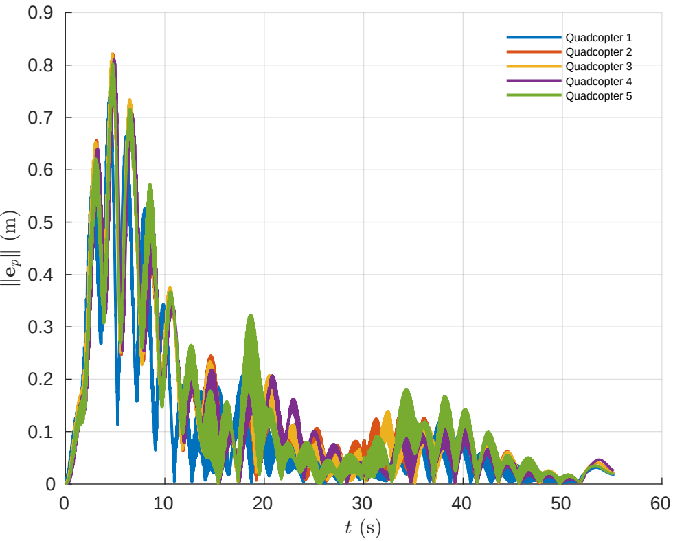
All Drones - 3D Position Error vs Time
