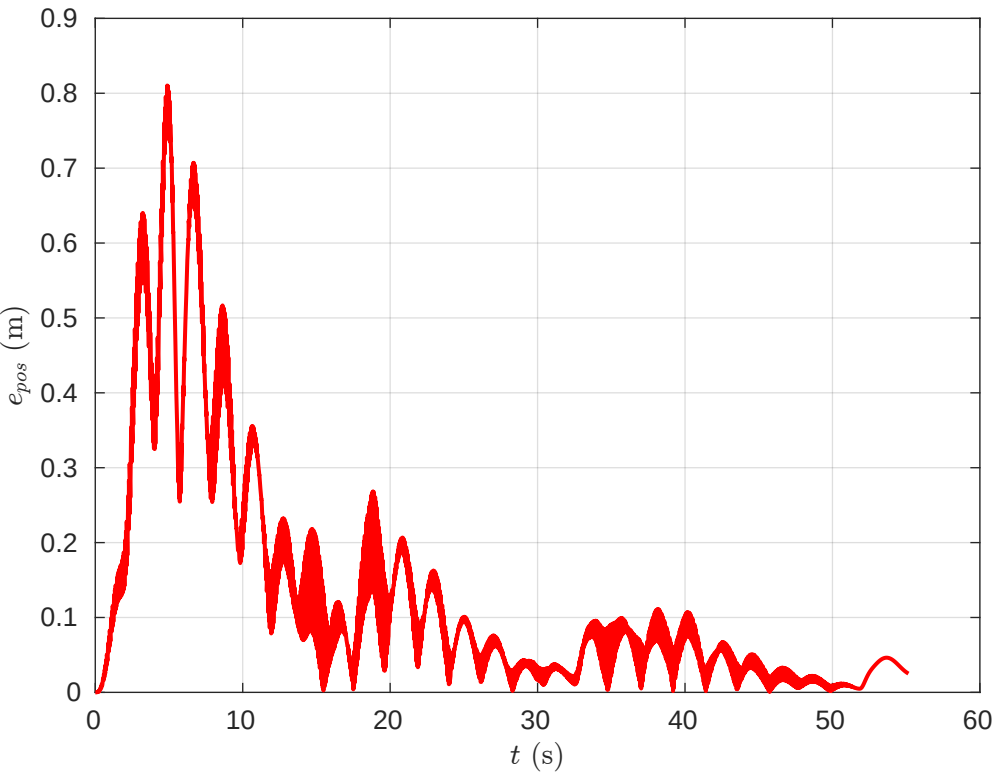
Drone 4 - 3D Position Error vs Time
