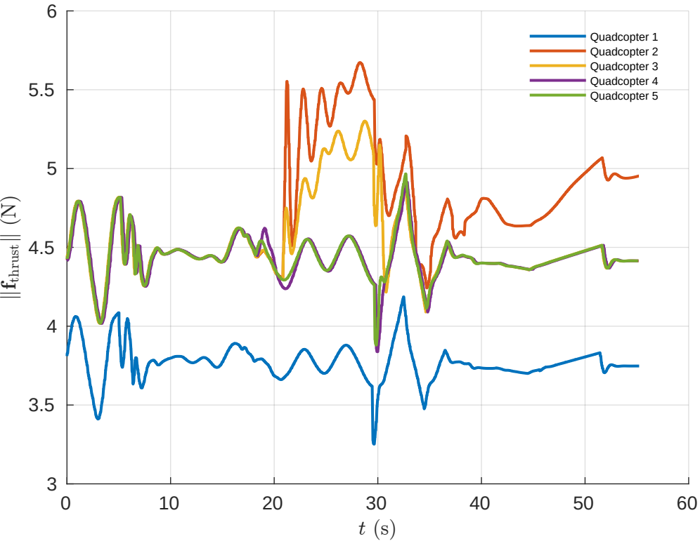
All Drones - Thrust vs Time
