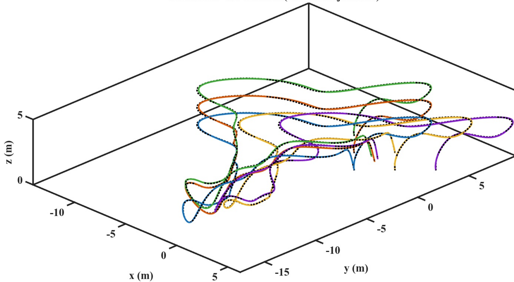
All Drones - 3D Position (Actual Trajectories)
