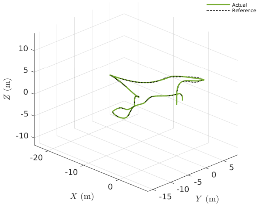
Drone 5 - 3D Position + Waypoints
