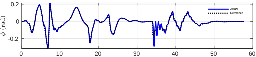
Drone 5 - Euler Angles vs Time
