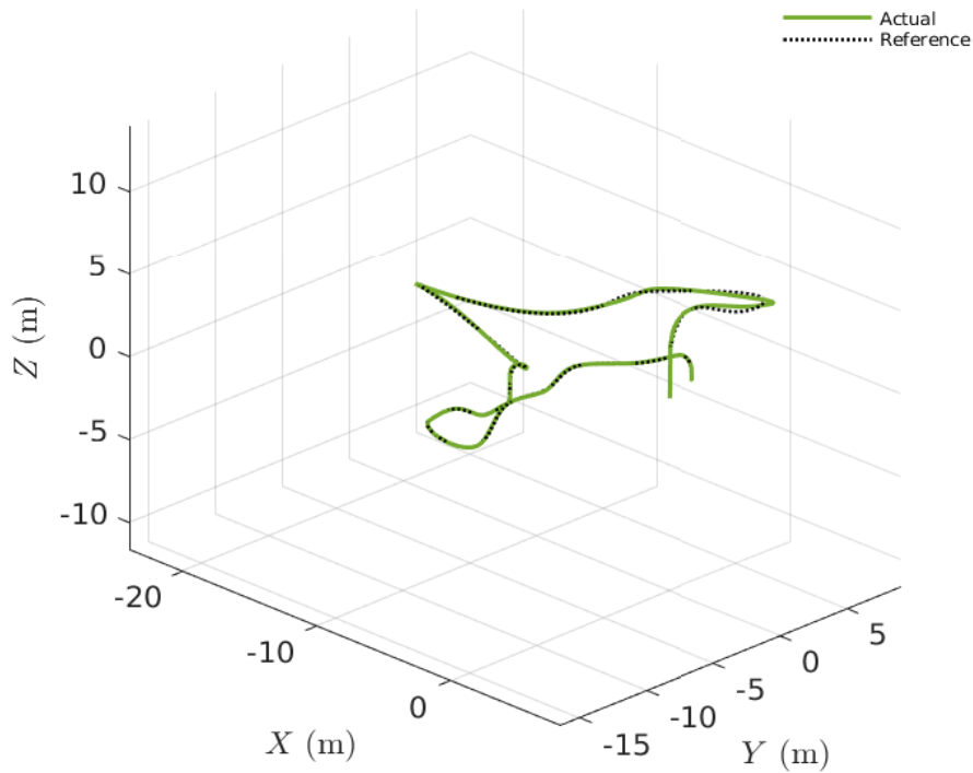
Drone 5 - 3D Position
