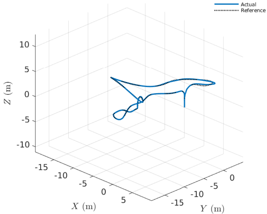
Drone 1 - 3D Position
