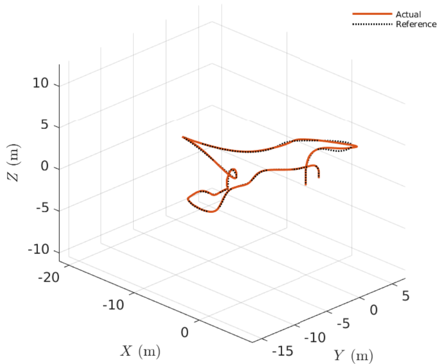
Drone 2 - 3D Position
