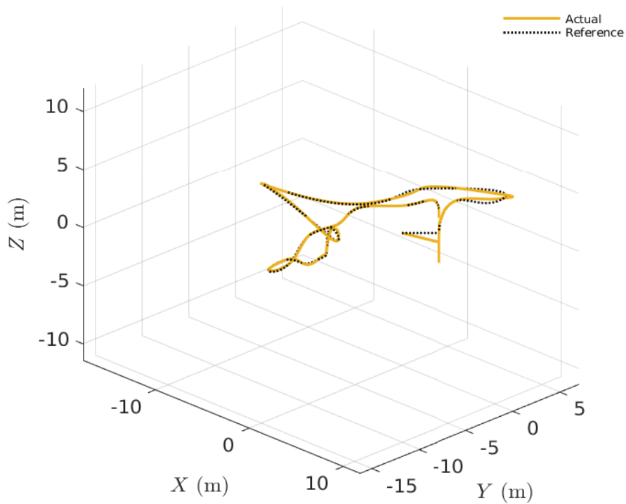
Drone 3 - 3D Position + Waypoints
