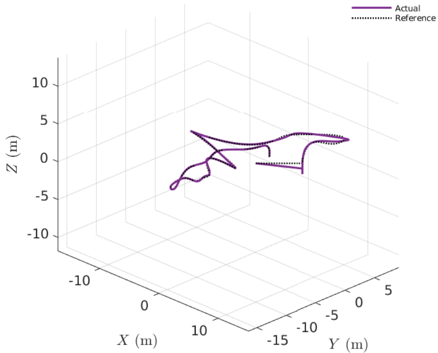
Drone 4 - 3D Position
