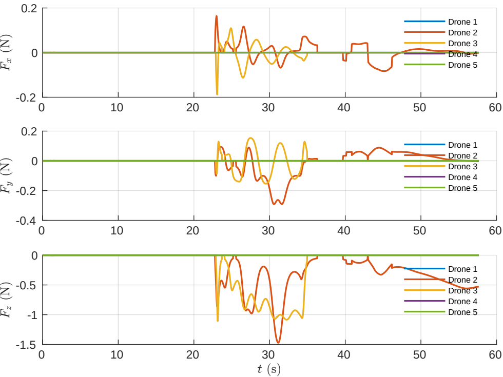
All Drones - Disturbance Forces vs Time
