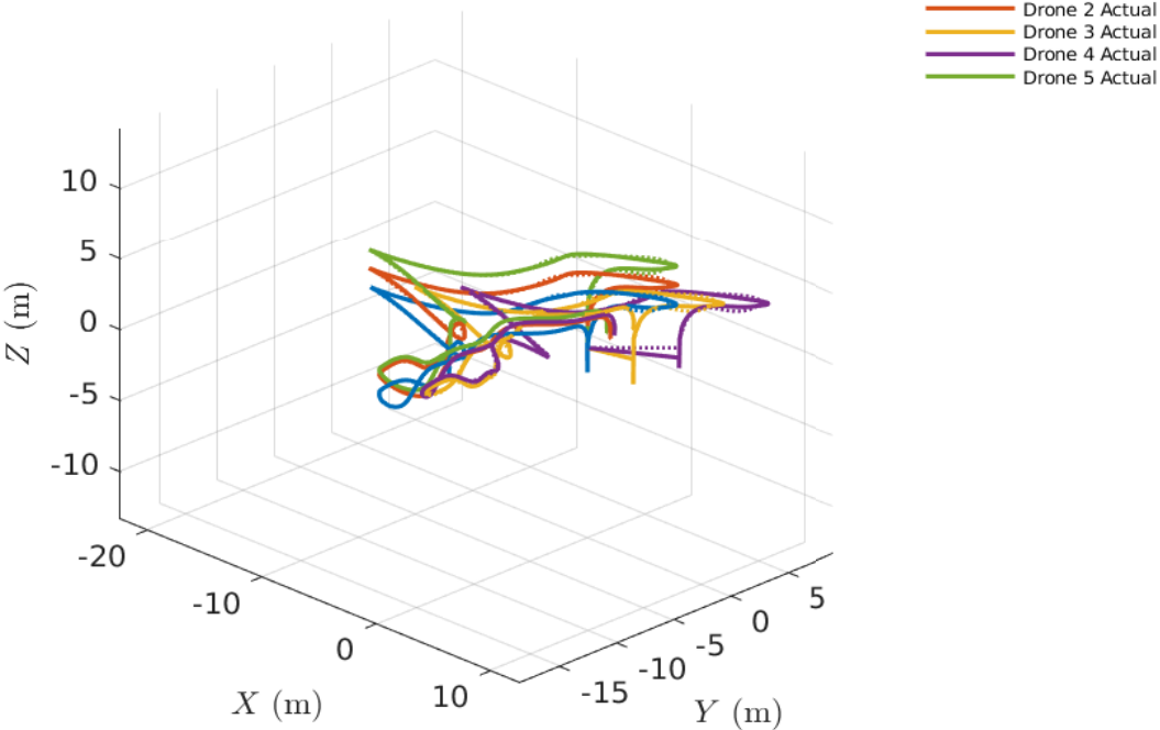
All Drones - 3D Position (Actual Trajectories)
