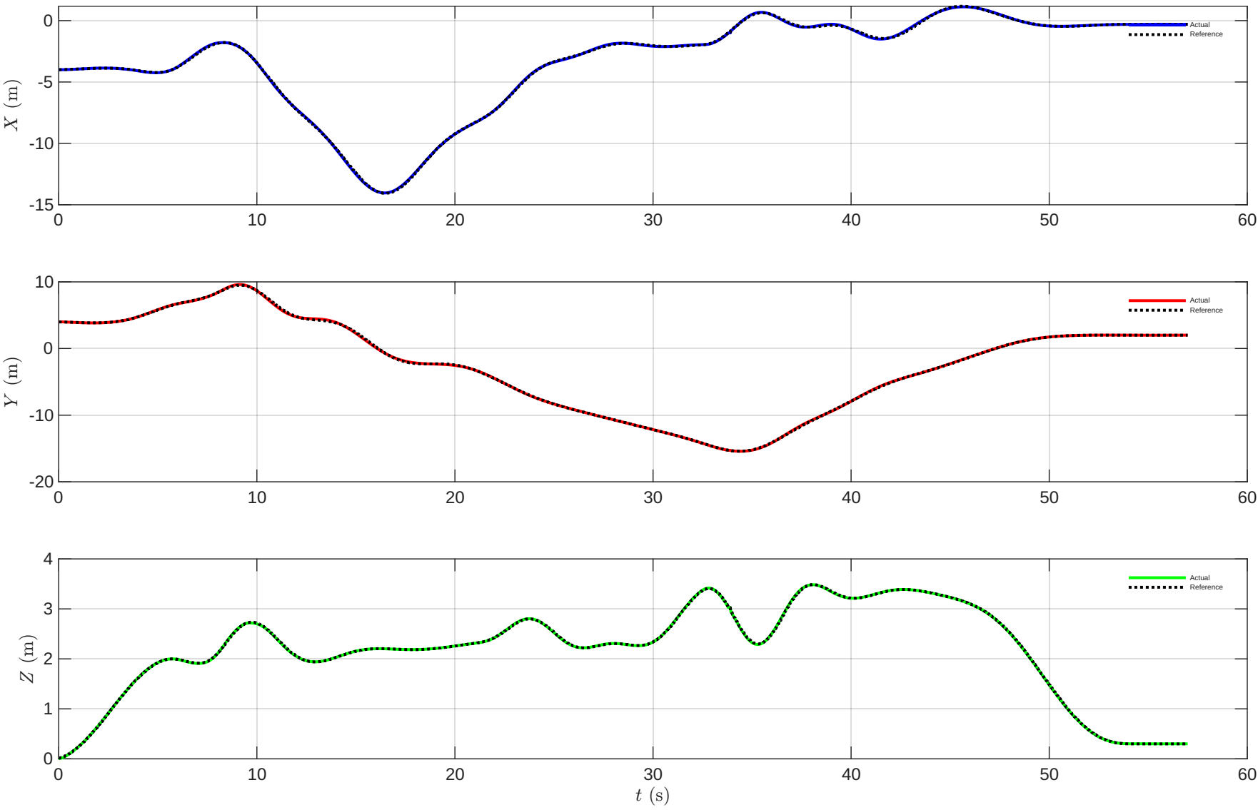
Drone 5 - Position vs Time
