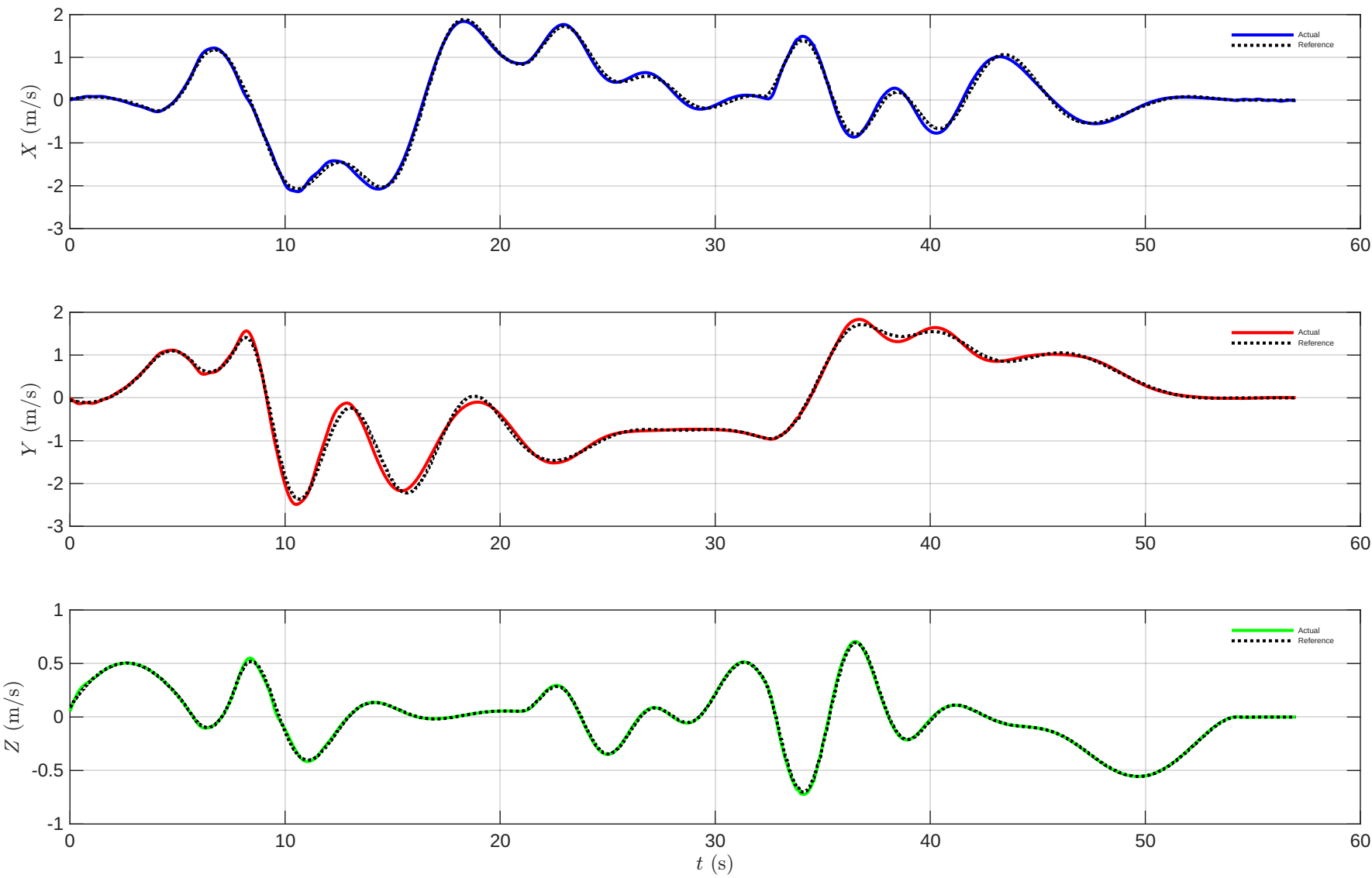
Drone 5 - Velocity vs Time
