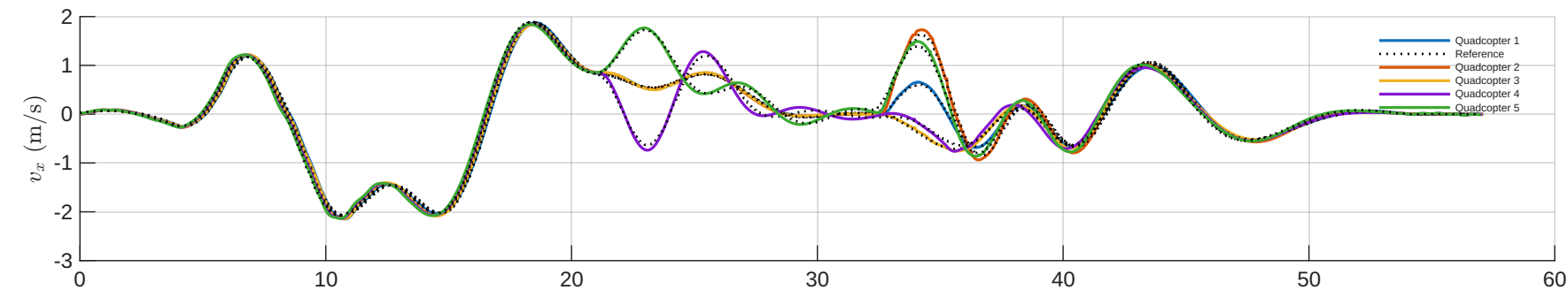
All Drones - Velocity (Actual vs Reference) vs Time
