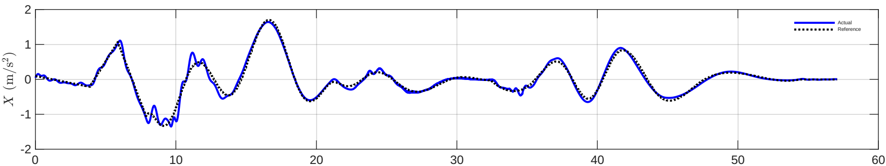
Drone 3 - Acceleration vs Time
