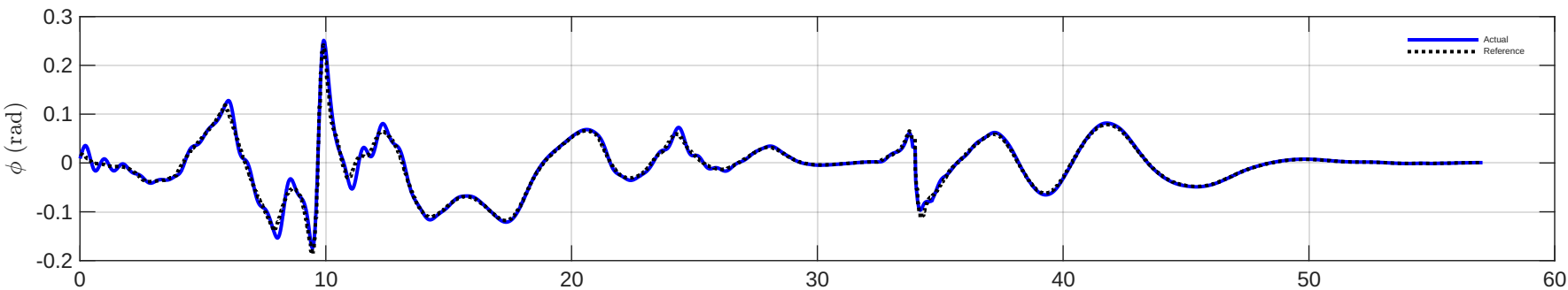
Drone 3 - Euler Angles vs Time
