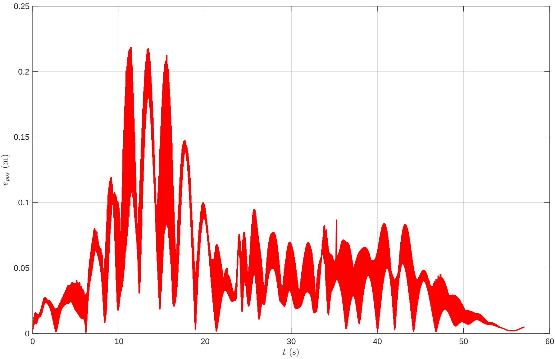
Drone 3 - 3D Position Error vs Time
