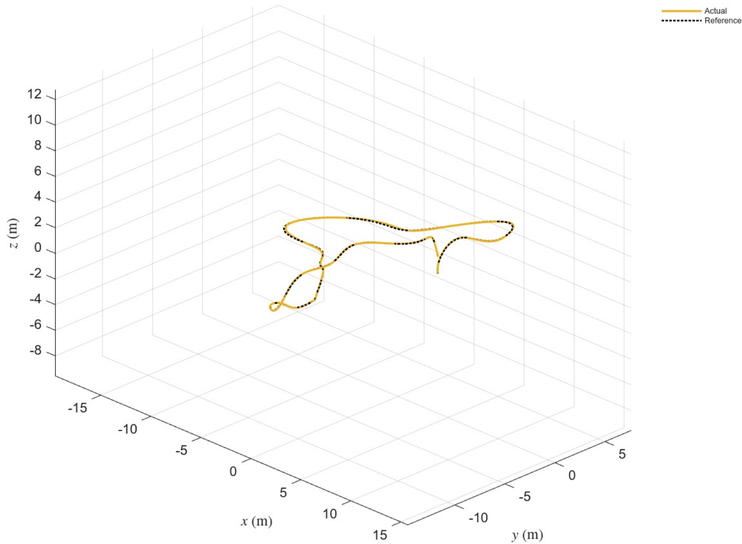
Quadcopter 3 - 3D Position + Waypoints
