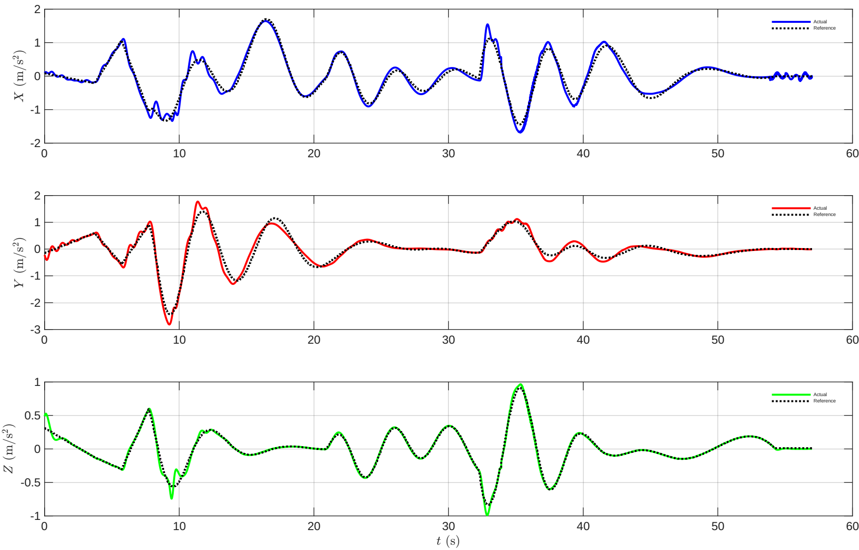
Drone 5 - Acceleration vs Time
