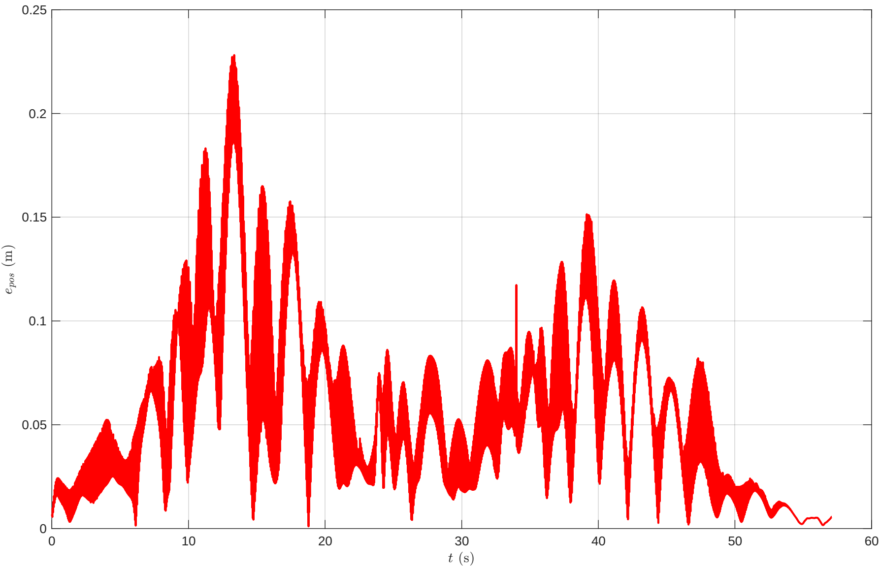
Drone 2 - 3D Position Error vs Time
