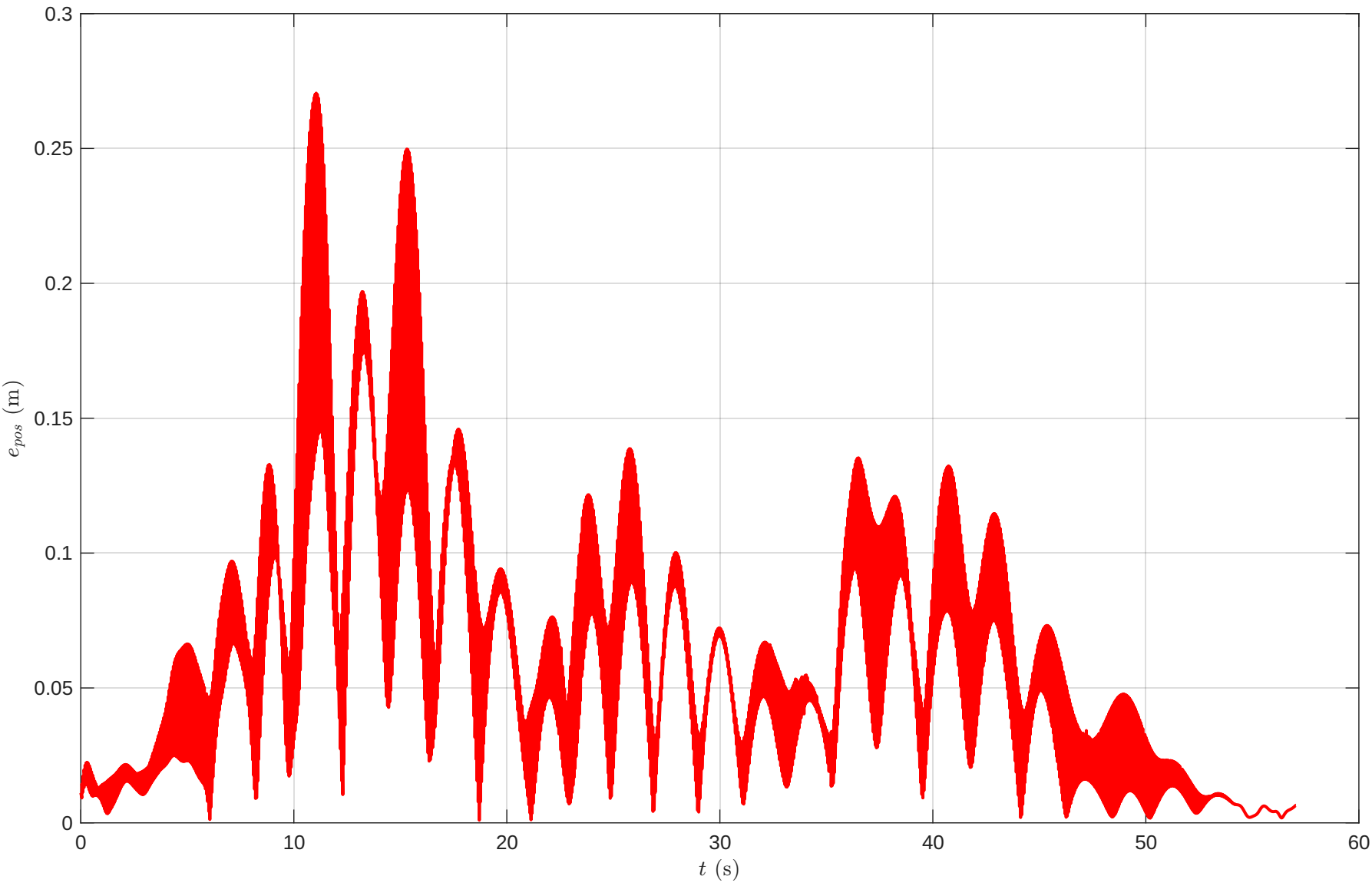
Drone 4 - 3D Position Error vs Time
