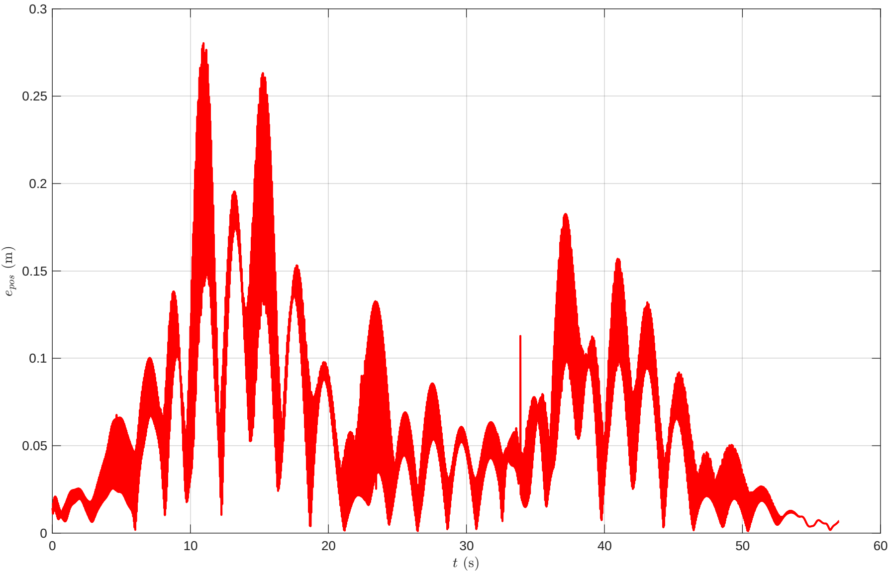
Drone 5 - 3D Position Error vs Time
