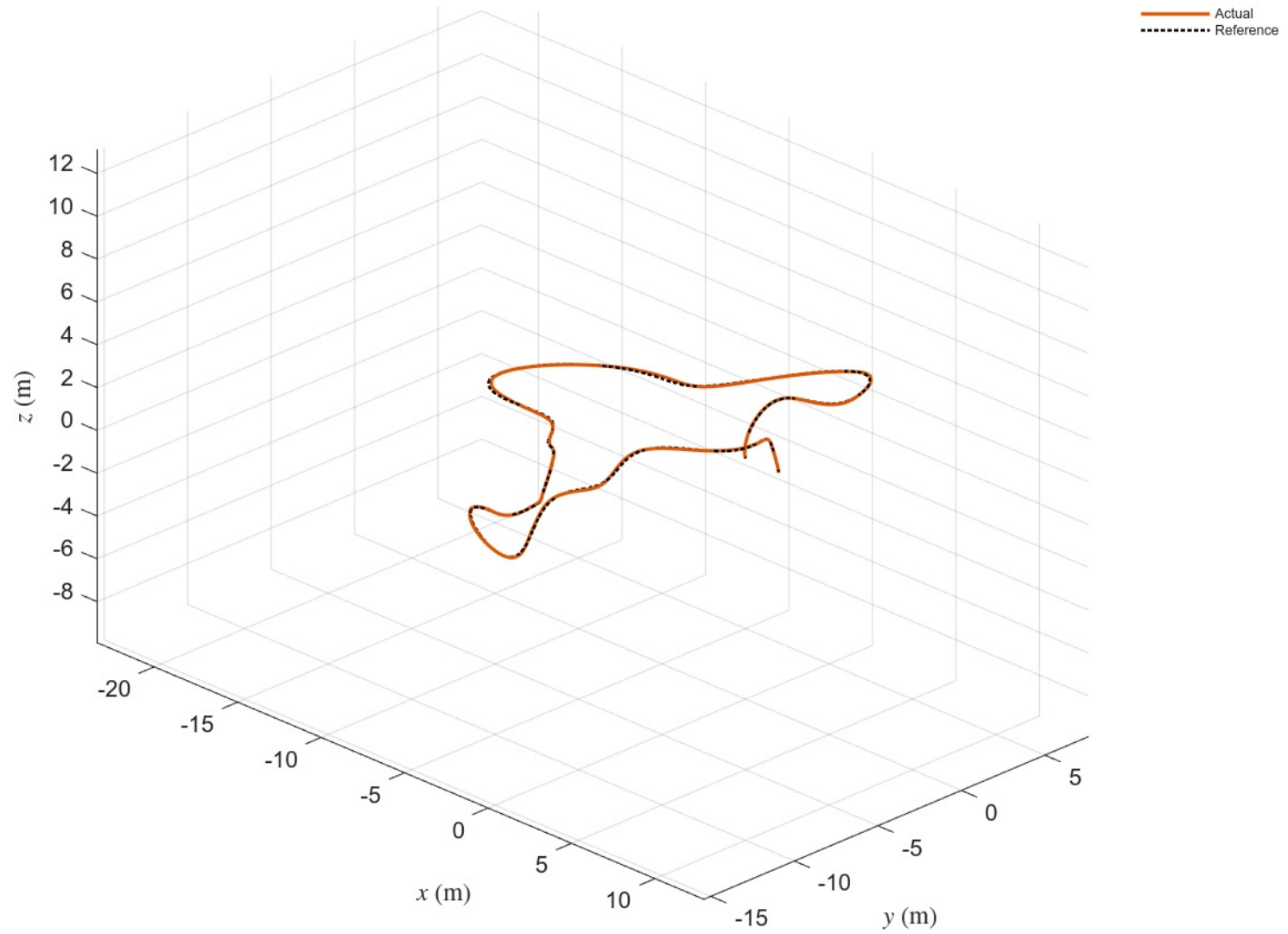
Quadcopter 2 - 3D Position + Waypoints
