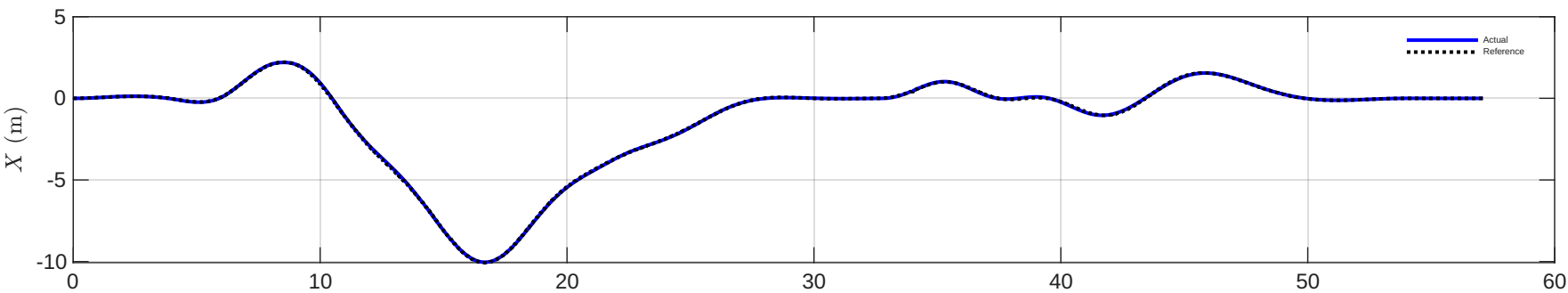
Drone 1 - Position vs Time
