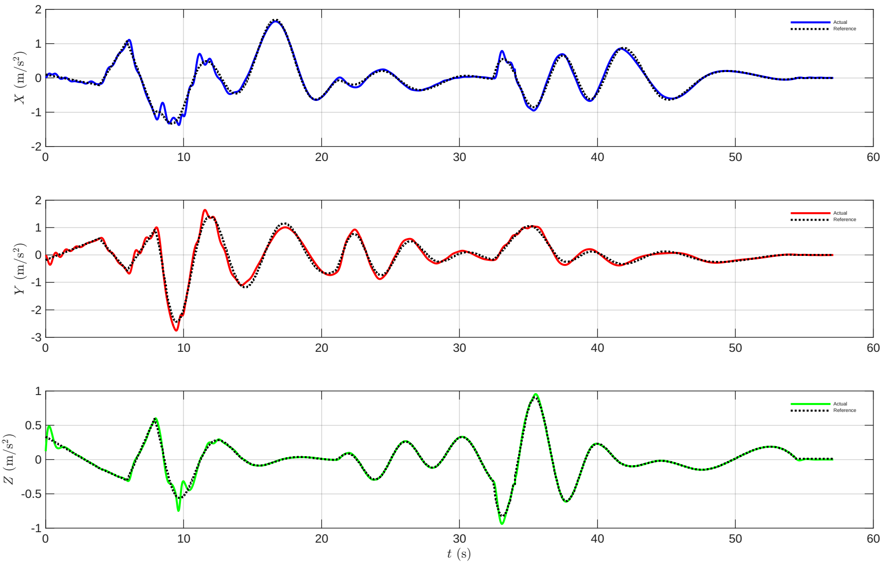
Drone 1 - Acceleration vs Time
