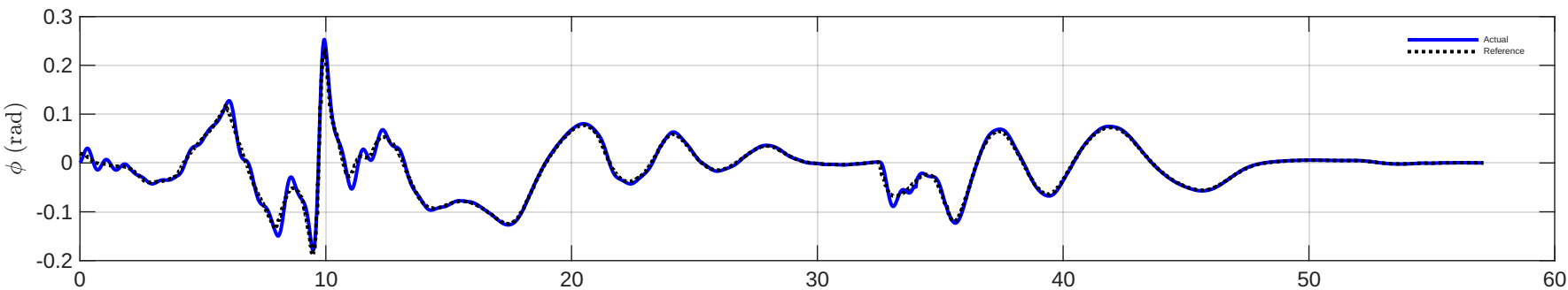
Drone 1 - Euler Angles vs Time
