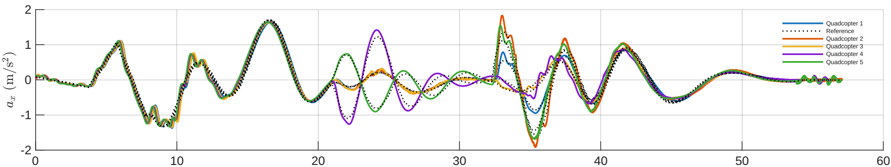
All Drones - Acceleration (Actual vs Reference) vs Time
