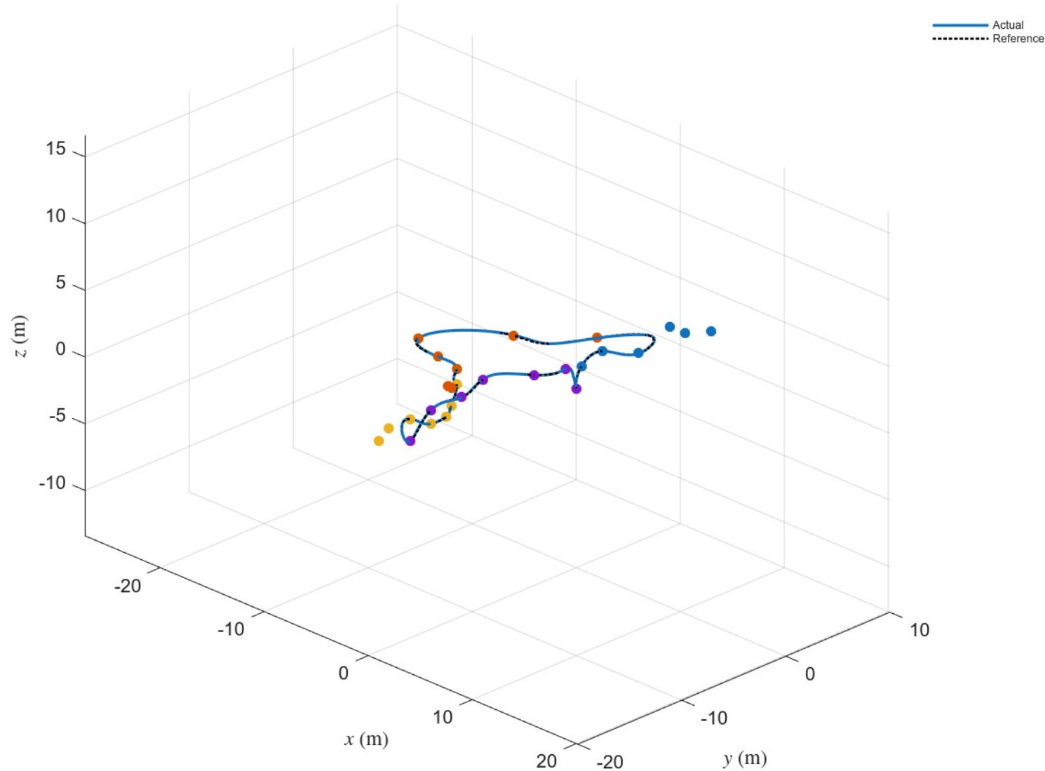
Quadcopter 1 - 3D Position + Waypoints
