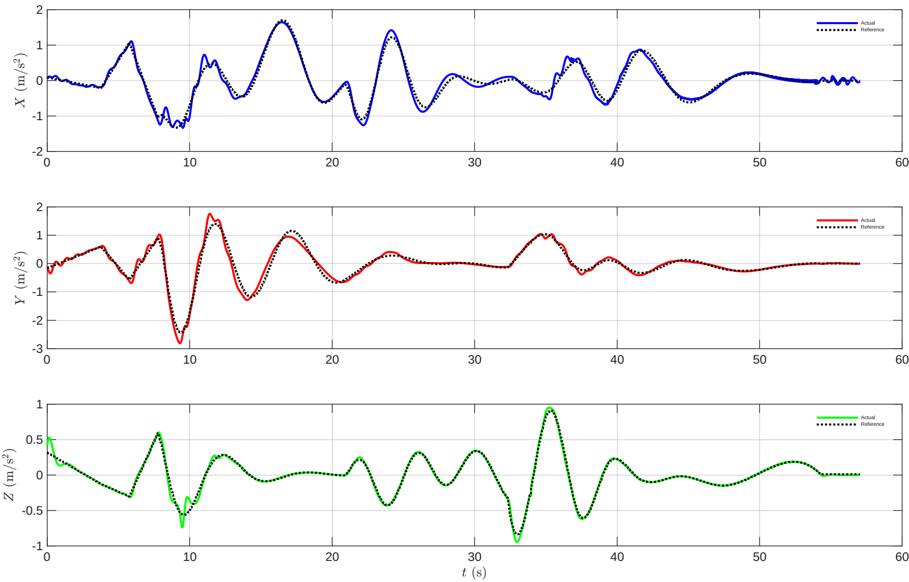
Drone 4 - Acceleration vs Time
