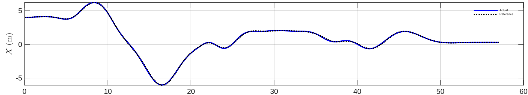
Drone 4 - Position vs Time
