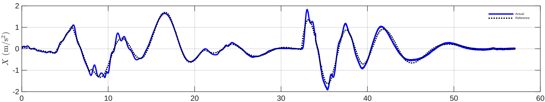
Drone 2 - Acceleration vs Time
