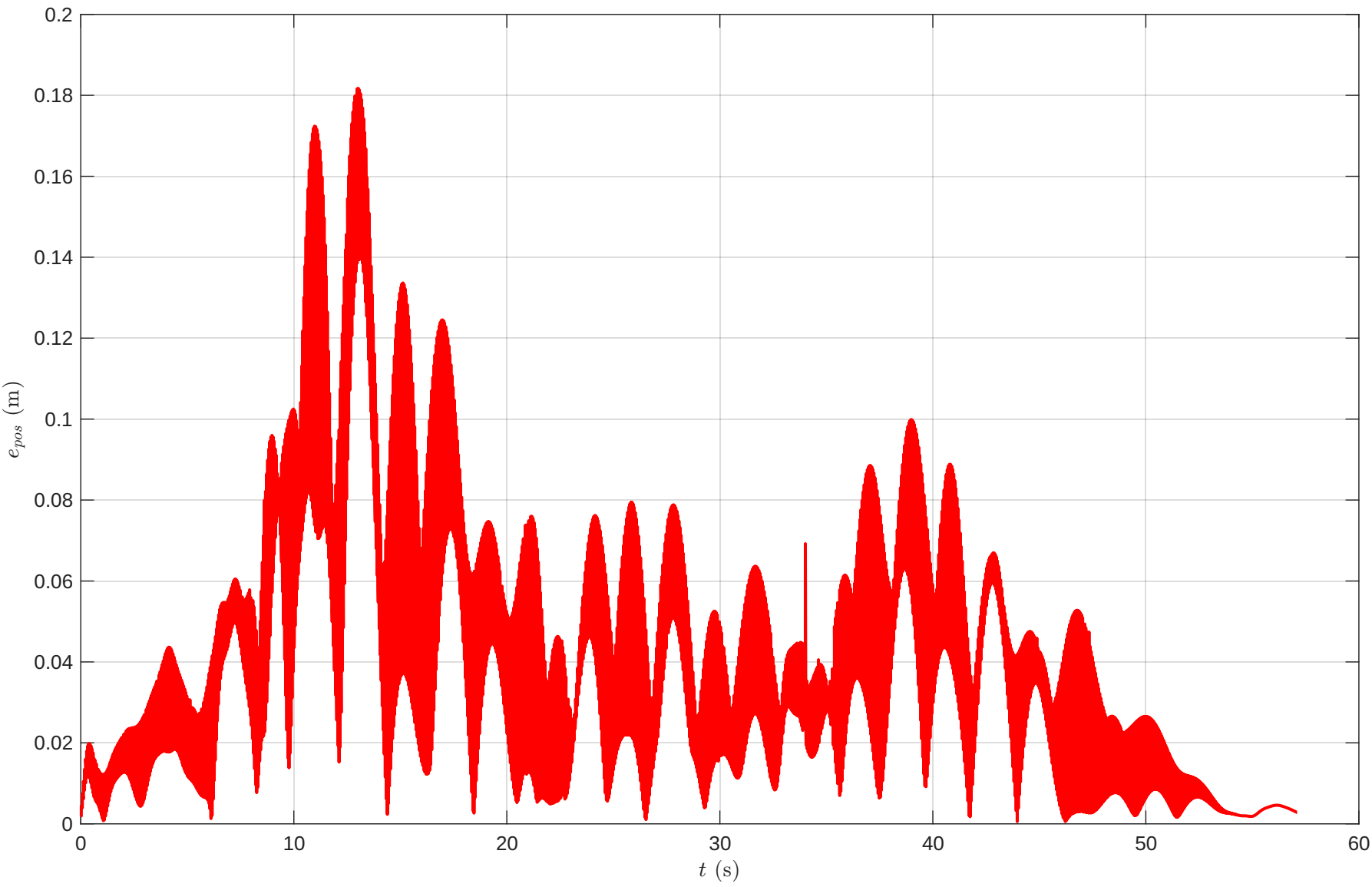
Drone 1 - 3D Position Error vs Time
