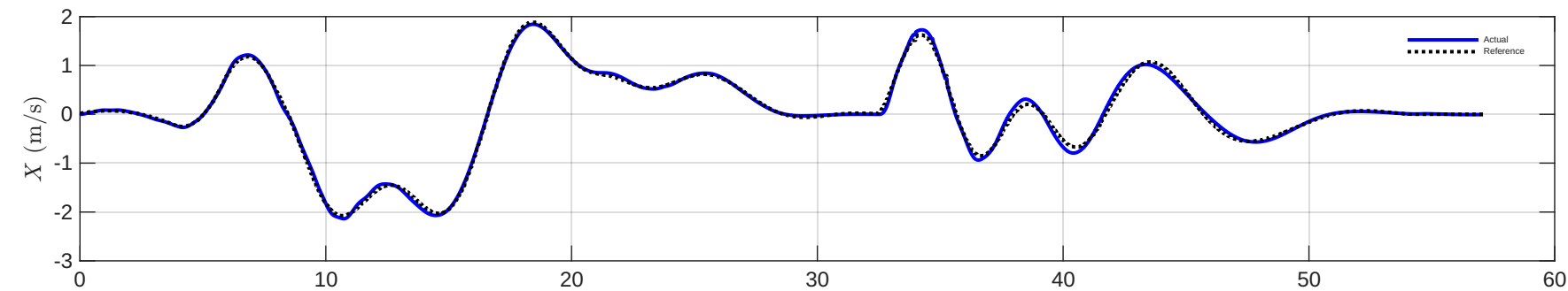
Drone 2 - Velocity vs Time
