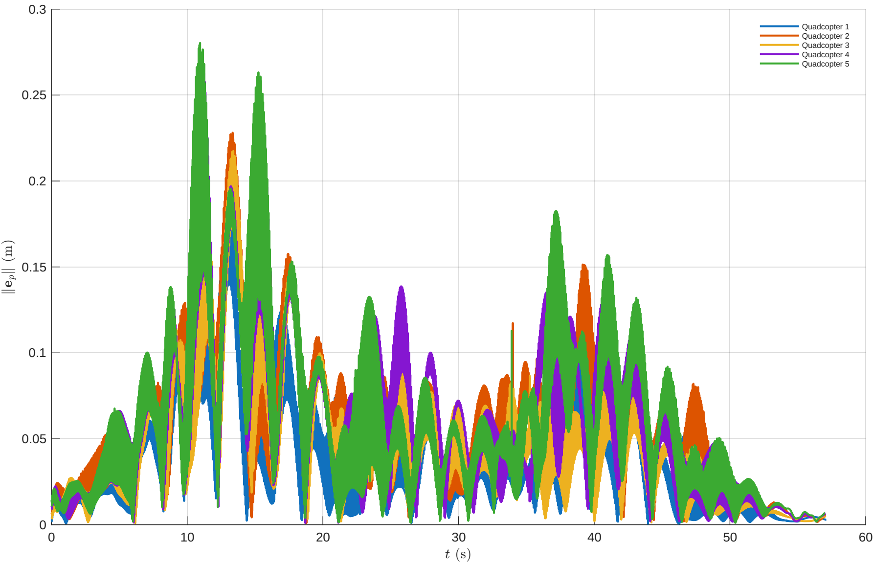
All Drones - 3D Position Error vs Time
