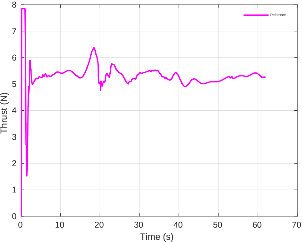
Drone 4 - Thrust vs Time
