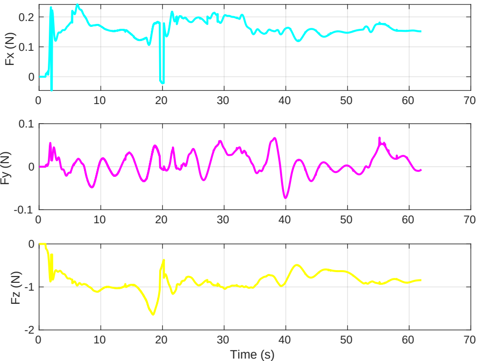
Drone 4 - Disturbance Force vs Time
