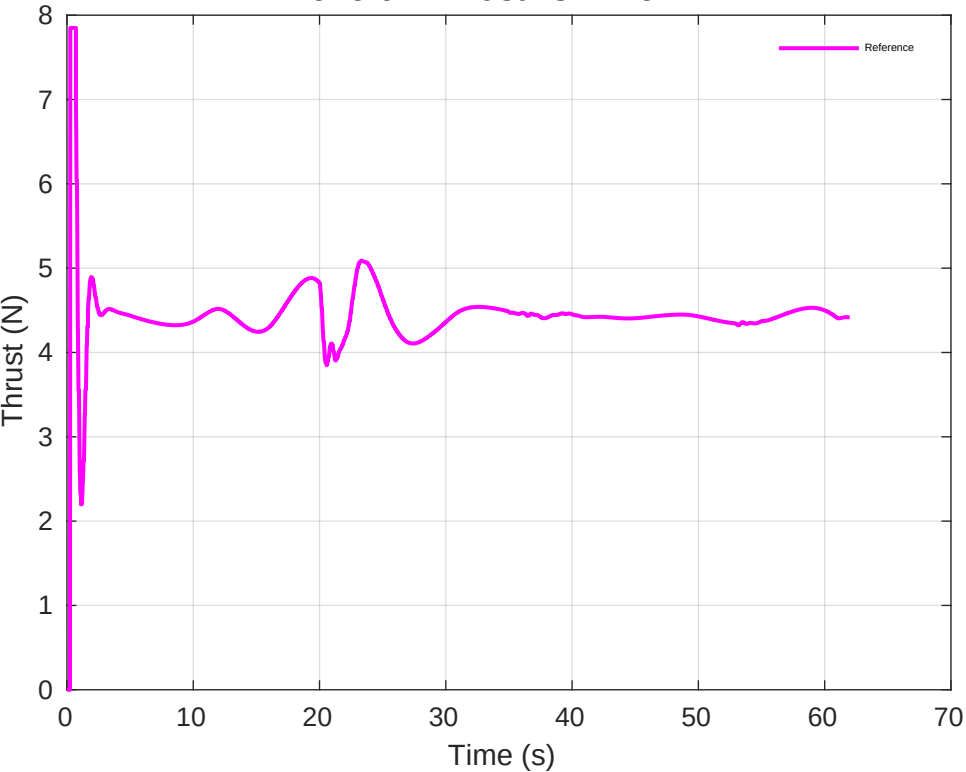
Drone 6 - Thrust vs Time
