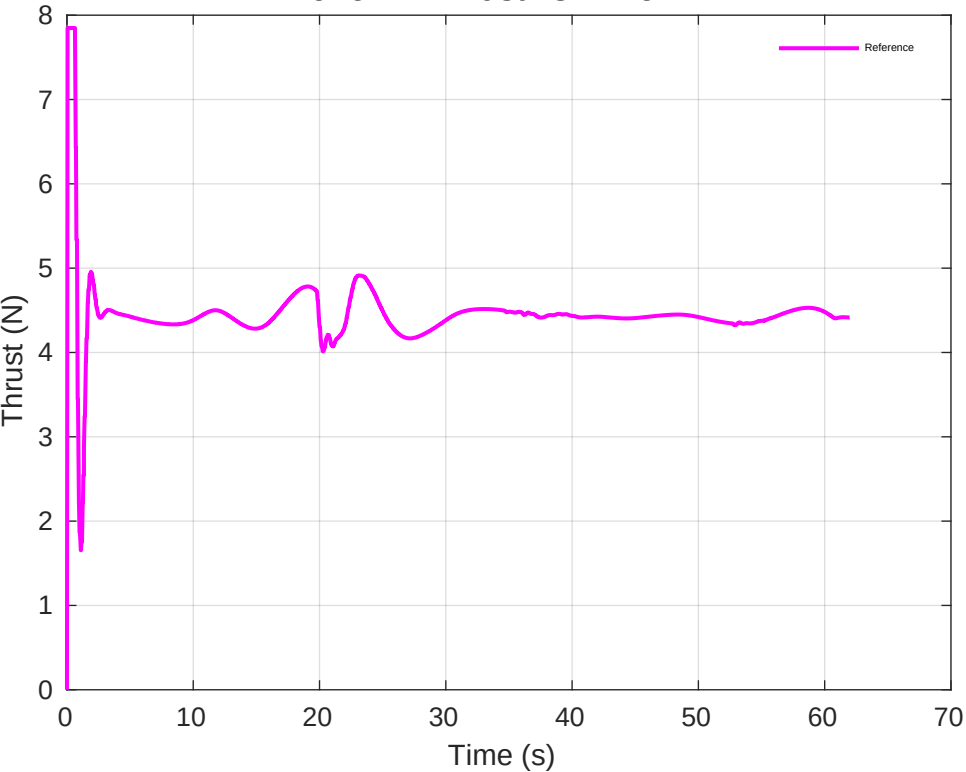
Drone 1 - Thrust vs Time
