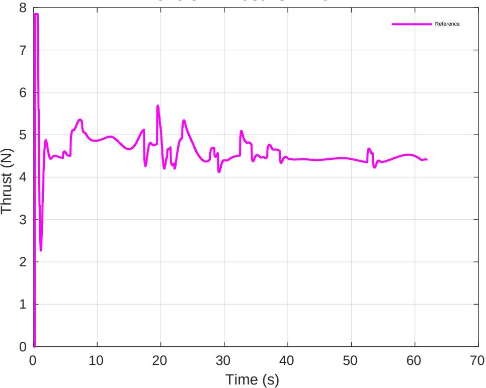
Drone 5 - Thrust vs Time
