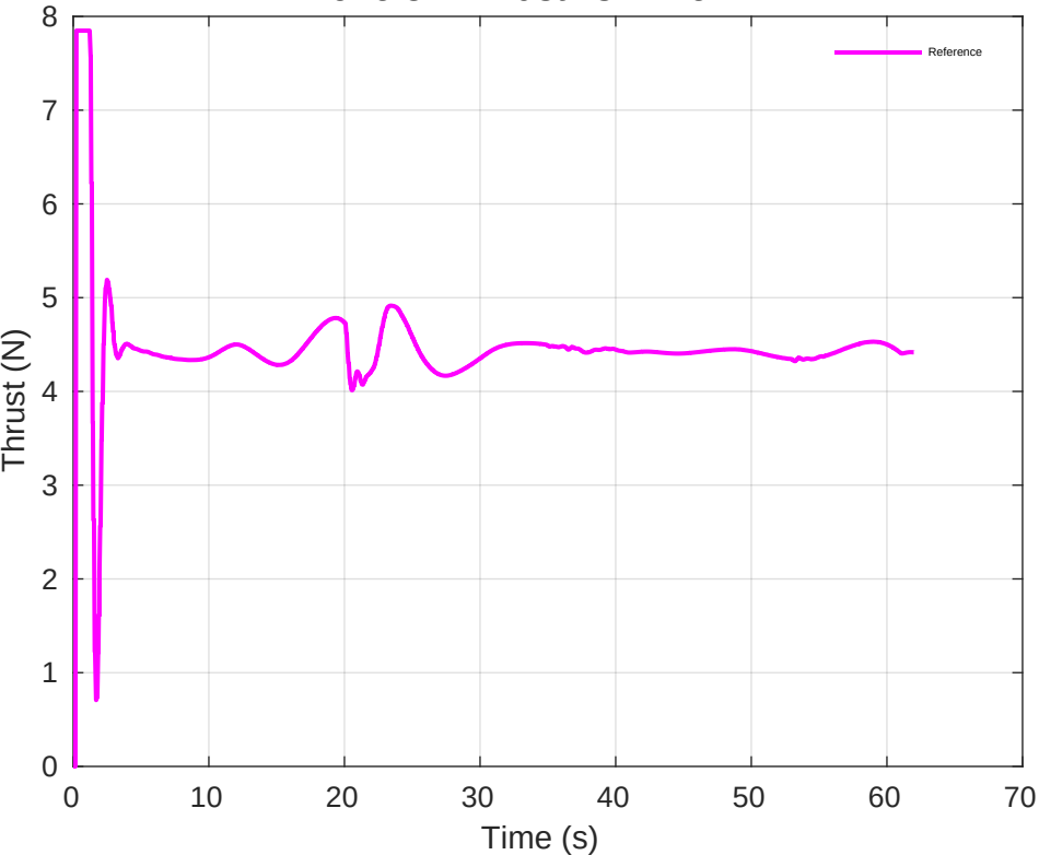
Drone 3 - Thrust vs Time
