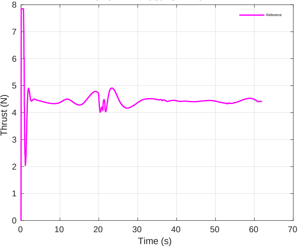
Drone 2 - Thrust vs Time
