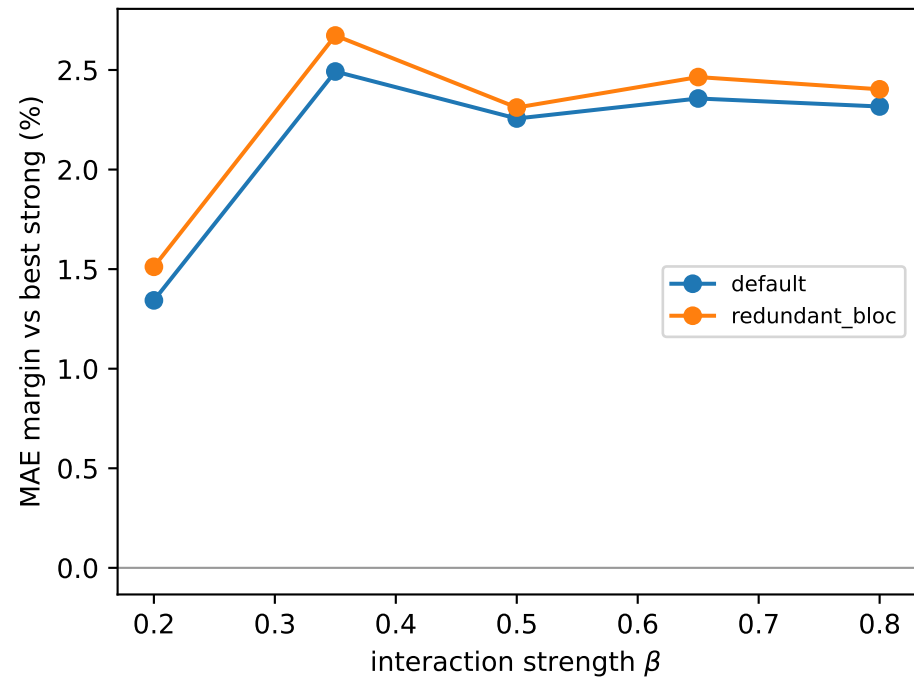
Robustness to \beta
