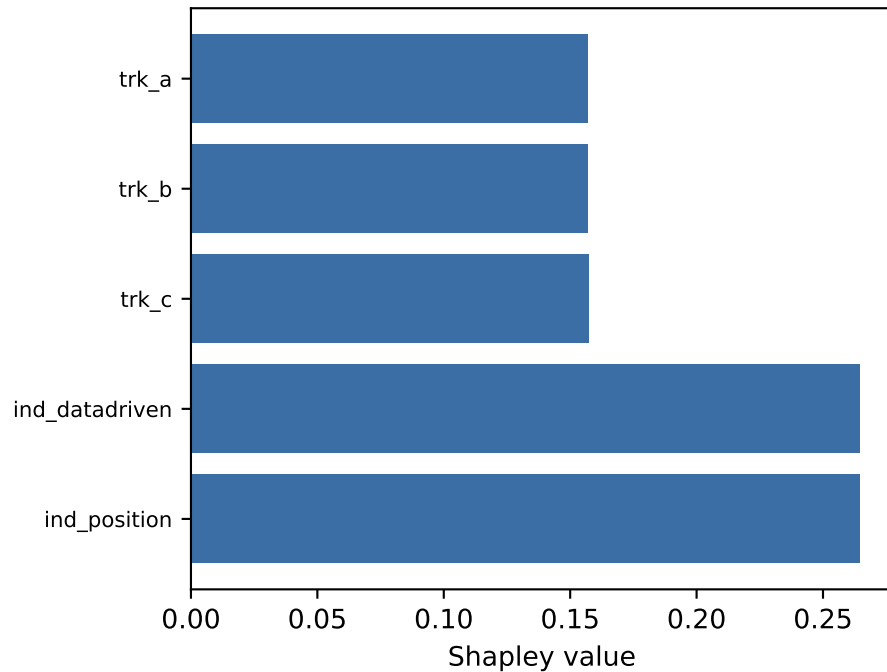
Source importance (Shapley)
