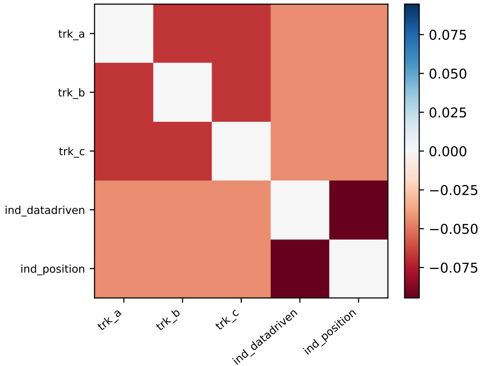
Interaction indices m_{st} (negative = redundant)
