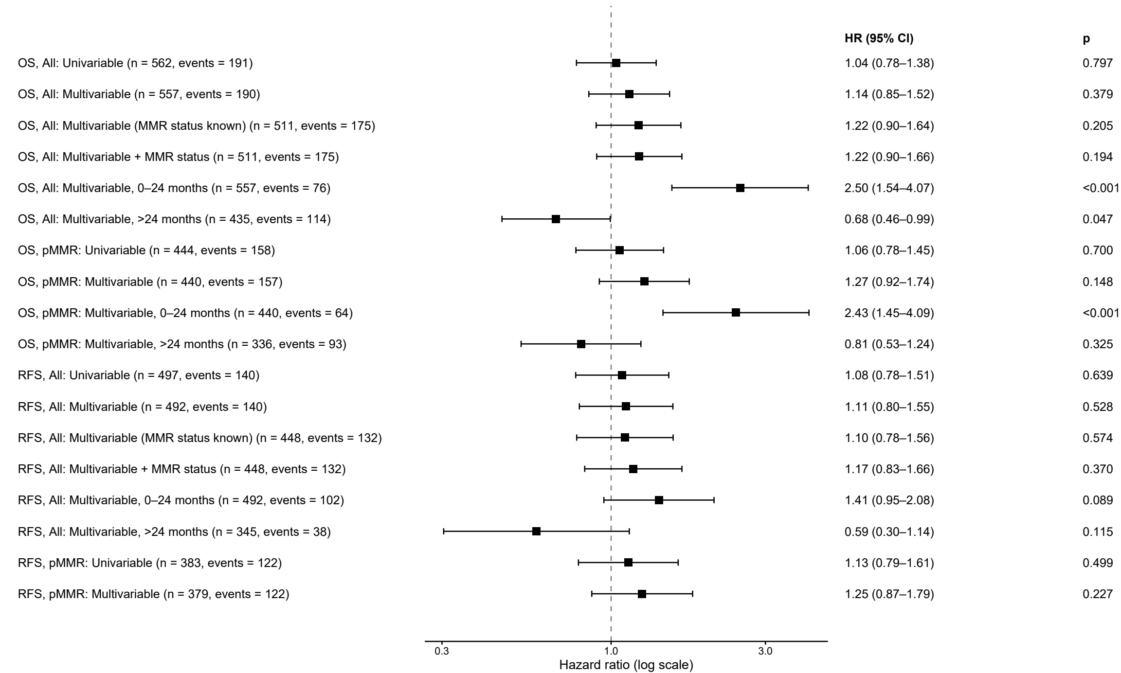
MS4A1 expression (High vs Low) — GSE39582 (CIT, colon) Probe 228592_at; multivariable models adjusted for age (per 10 years), sex and pathologic stage
