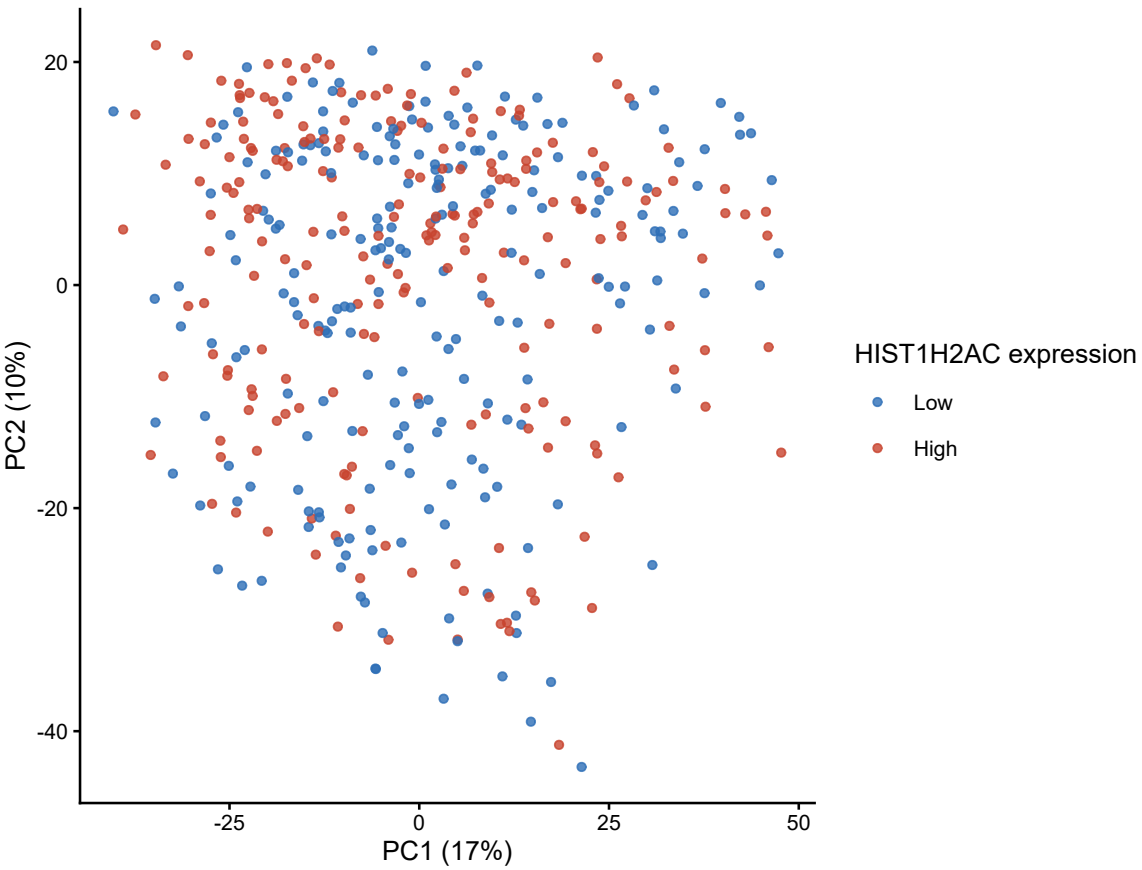
PCA of variance-stabilized expression — TCGA-COAD
