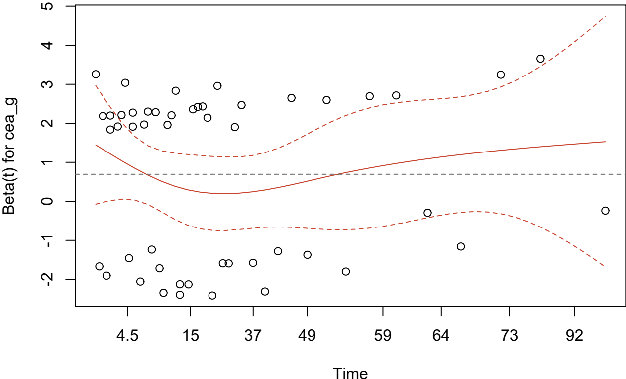
TP53 — multivariable: cea_g (p = 0.976)
