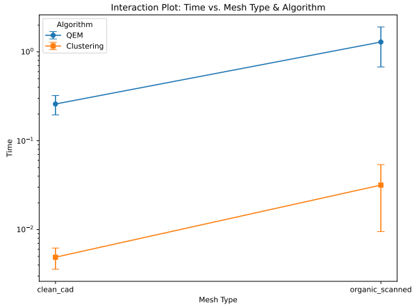
Figure 3: Interaction Plot for CPU Time. QEM is significantly more sensitive to mesh complexity than Clustering.
