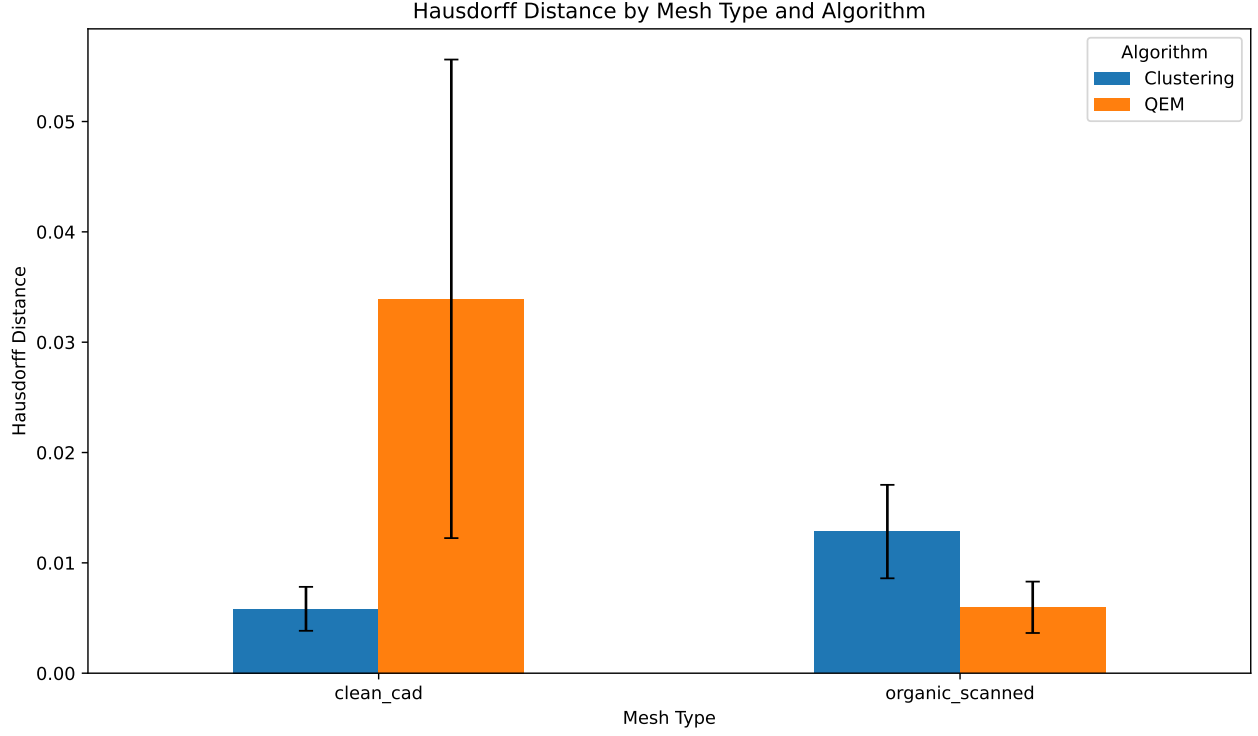
Figure 4: Mean Hausdorff Distance (Error) by Algorithm and Mesh Type. Error bars represent 95% Confidence Intervals. Lower is better. (Double-column view for detail)
