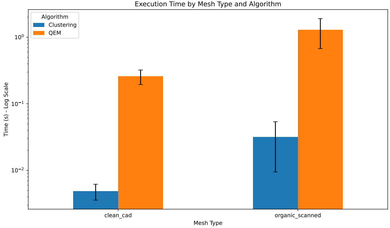
Figure 2: Mean CPU Time by Algorithm and Mesh Type. Error bars represent 95% Confidence Intervals. (Double-column view for detail)
