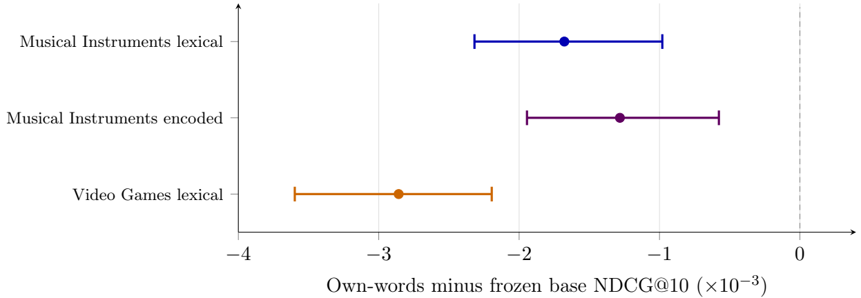
Figure 3: Exploratory own-words wording arm against the frozen behavioural base on the full test splits. Points are paired NDCG@10 differences; lines are user-cluster bootstrap 95% intervals. Lexical retrieval was measured in both categories; encoded retrieval was measured only in Musical Instruments. Both test periods had already been opened by earlier work, so these intervals describe regressions on those cohorts rather than independent confirmation.
