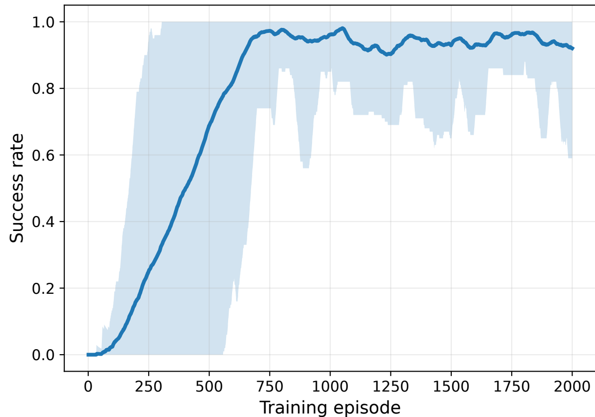
(a) PPO success rate across seeds
