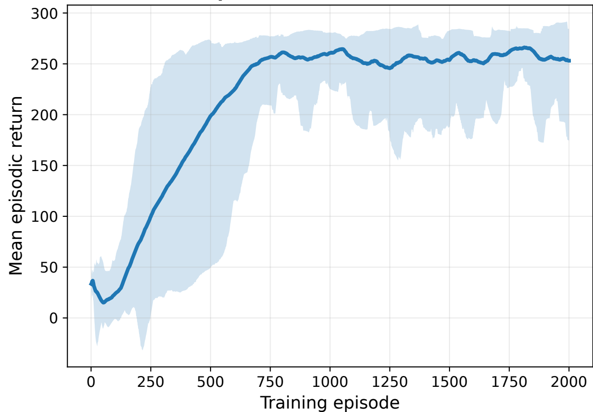
(b) PPO mean episodic return across seeds
