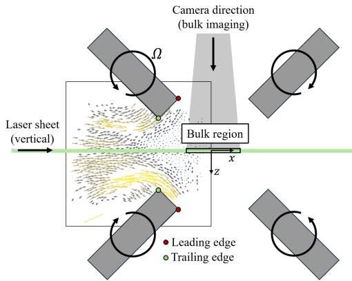
FIG. 10. Schematic of the viewing area in the horizontal plane with respect to the position of the blades, as well as laser sheet and camera directions during bulk imaging.
