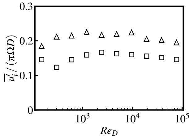
FIG. 3. Spatially averaged root-mean-square velocity fluctuations in the bulk, normalized by \pi \Omega D , versus the blade Reynolds number Re_D . Triangles denote the horizontal component ( u ); squares denote the vertical component ( v ).
