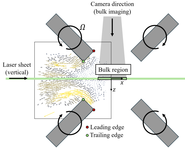
FIG. 9. Schematic of the viewing area in the horizontal plane with respect to the position of the blades, as well as laser sheet and camera directions during bulk imaging.
