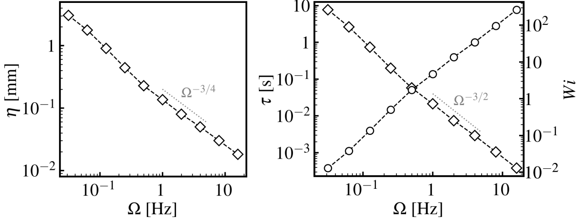
FIG. 4. Kolmogorov length scale as a function of rotation rate (left). Kolmogorov time scale and estimated Weissenberg numbers (square and circular markers respectively) (right).
