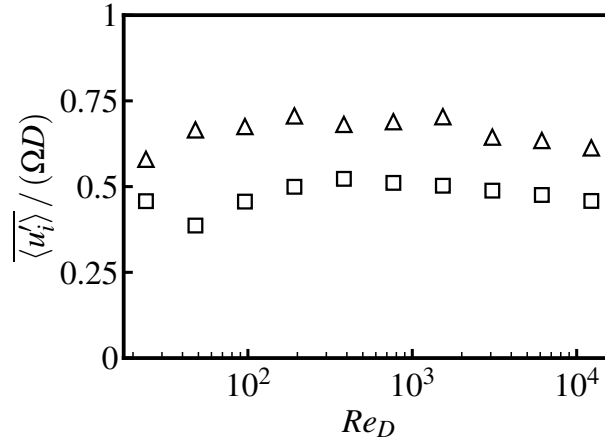
FIG. 3. Spatially averaged velocity fluctuation RMS in the bulk as a function of rotation rate of the agitator blades.
