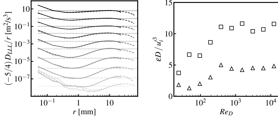
FIG. 4. Normalized third-order structure function for different rotation rates. Darker lines represent a higher rotation rate (a). Dissipation rate as a function of the blade Reynolds number (b).
