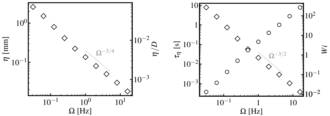
FIG. 5. Kolmogorov length scale as a function of rotation rate (left). Kolmogorov time scale and estimated Weissenberg numbers (square and circular markers respectively) (right).
