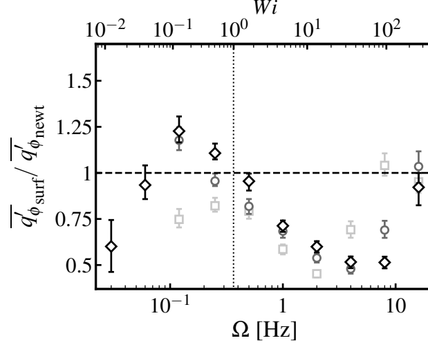
FIG. 11. Ratio of spatially averaged velocity fluctuation RMS (phase-locked) between the surfactant and Newtonian cases. Darker markers indicate higher solution concentration, with the squares denoting 33 ppm, circles denoting 50 ppm and diamonds denoting 100 ppm solution.
