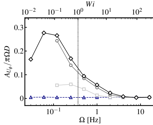
FIG. 9. Normalized amplitude of the spatially averaged, phase-locked horizontal component of the mean flow as a function of rotation rate. Grayscale curves denote surfactant solutions with darker markers indicating higher solution concentration. Squares denoting 33 ppm, circles denoting 50 ppm and diamonds denoting 100 ppm solution. Blue line with triangle markers denote Newtonian flow.
