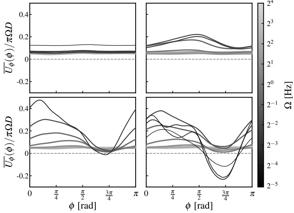
FIG. 8. Spatially averaged horizontal mean flow component as a function of blade phase for (a) Newtonian, (b) 33 ppm, (c) 50 ppm and (d) 100 ppm solutions. Positive value refers to inward motion (towards the stagnation point), while a negative value indicates flow reversal.
