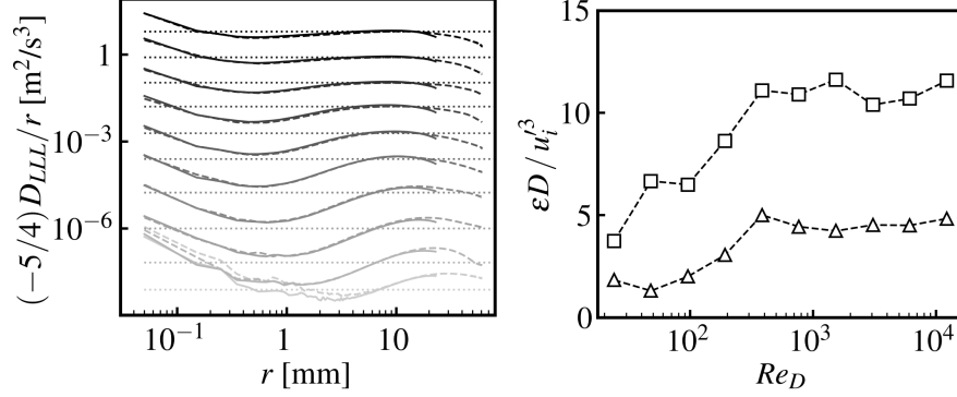
FIG. 4. Normalized third-order structure function for different rotation rates. Darker lines represent a higher rotation rate (a). Dissipation rate as a function of the blade Reynolds number (b).
