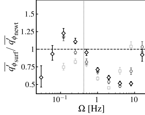
FIG. 11. Ratio of spatially averaged velocity fluctuation RMS (phase-locked) between the surfactant and Newtonian cases.
