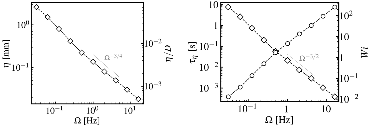
FIG. 5. Kolmogorov length scale as a function of rotation rate (left). Kolmogorov time scale and estimated Weissenberg numbers (square and circular markers respectively) (right).
