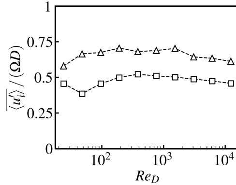
FIG. 3. Spatially averaged velocity fluctuation RMS in the bulk as a function of rotation rate of the agitator blades.
