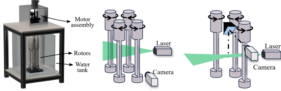
FIG. 1. Schematic (a) of the experimental device and zoomed-in views showing the laser sheet and camera orientations for the imaging of (b) the bulk and (c) the vicinity of the blades in the horizontal plane.
