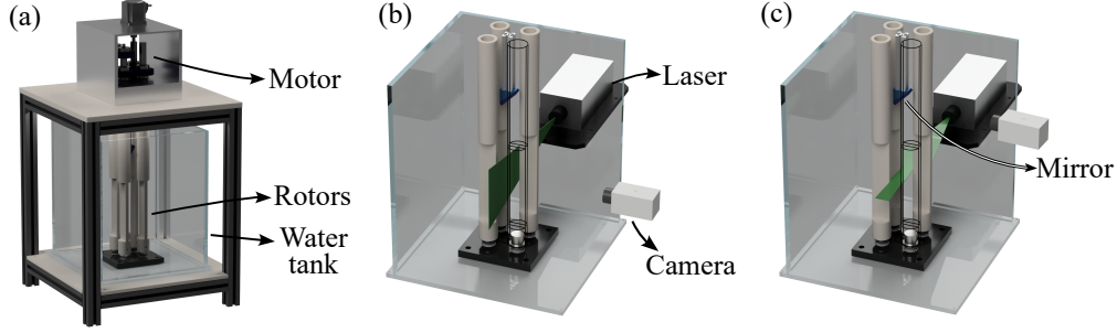
FIG. 1. Schematic (a) of the experimental device and zoomed-in views showing the laser sheet and camera orientations for the imaging of (b) the bulk and (c) the vicinity of the blades in the horizontal plane.
