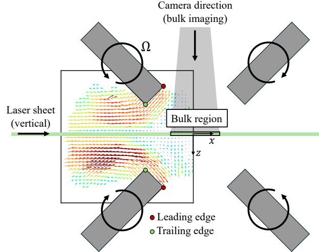
FIG. 2. Schematic of the viewing area in the horizontal plane with respect to the position of the blades, as well as laser sheet and camera directions during bulk imaging.
