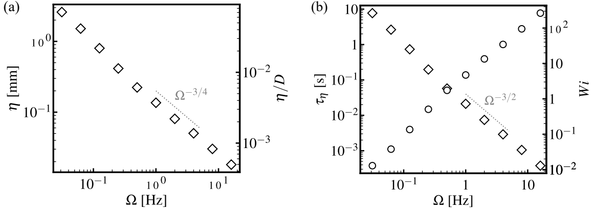
FIG. 5. (a) Kolmogorov length scale \eta versus blade rotation rate \Omega ; diamonds denote the estimates and the dotted line indicates the \Omega^{-3/4} scaling. (b) Kolmogorov time scale \tau_\eta (diamonds, left axis) and estimated Weissenberg number Wi (circles, right axis) versus \Omega . The dotted line indicates the \Omega^{-3/2} scaling; Wi is calculated using \tau_s = 0.1 s.
