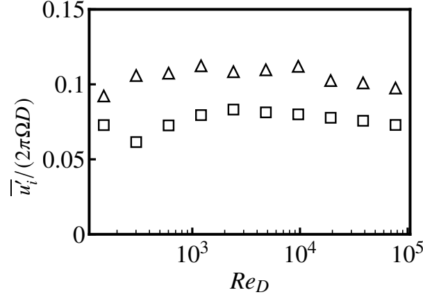
FIG. 3. Spatially averaged root-mean-square velocity fluctuations in the bulk, normalized by 2\pi\Omega D , versus the blade Reynolds number Re_D . Triangles denote the horizontal component ( u ); squares denote the vertical component ( v ).
