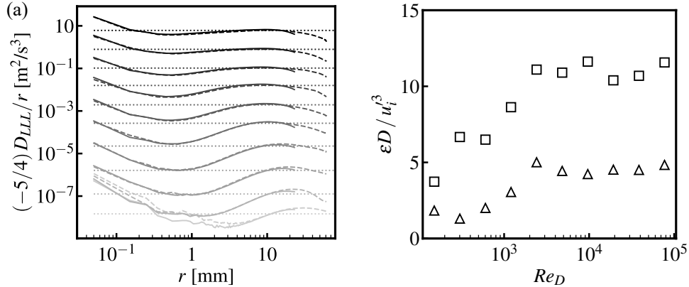
FIG. 4. (a) Compensated longitudinal third-order structure function, -5D_{LLL}^{(i)}(r)/(4r) , versus separation r for the Newtonian cases. Solid and dashed curves correspond to the two measured directions; darker curves indicate higher blade rotation rates. Dotted horizontal lines show the dissipation estimates obtained by averaging over 3 \leq r \leq 20 mm. (b) Dimensionless dissipation estimates, \varepsilon_i D / \overline{u_i'}^3 , versus blade Reynolds number Re_D . Triangles denote the horizontal direction ( i = x ); squares denote the vertical direction ( i = y ).
