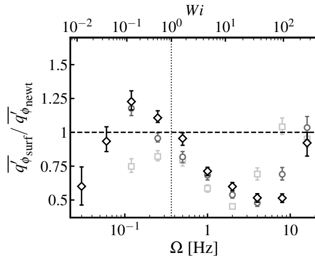
FIG. 11. Ratio of spatially averaged, phase-corrected velocity fluctuation RMS \overline{q'_\phi} between the surfactant and Newtonian cases. Darker markers indicate higher solution concentration, with the squares denoting 33 ppm, circles denoting 50 ppm and diamonds denoting 100 ppm solution.
