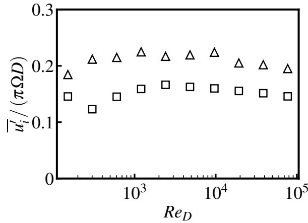
FIG. 3. Spatially averaged root-mean-square velocity fluctuations in the bulk, normalized by \pi \Omega D , versus the blade Reynolds number Re_D . Triangles denote the horizontal component ( u ); squares denote the vertical component ( v ).
