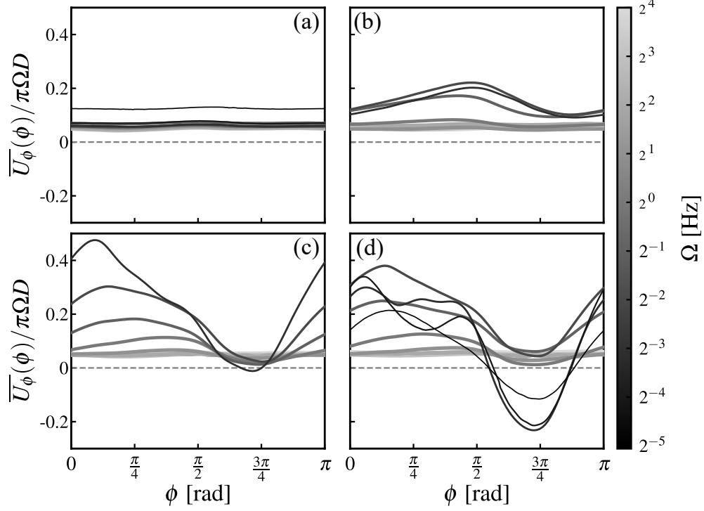
FIG. 8. Signed horizontal mean flow component \overline{U}_\phi , symmetry-enforced and spatially averaged over the left half of the measurement region, as a function of blade phase for (a) Newtonian, (b) 33 ppm, (c) 50 ppm and (d) 100 ppm solutions. Positive value refers to inward motion (towards the stagnation point), while a negative value indicates flow reversal.
