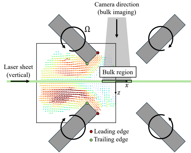
FIG. 2. Schematic of the viewing area in the horizontal plane with respect to the position of the blades, as well as laser sheet and camera directions during bulk imaging.
