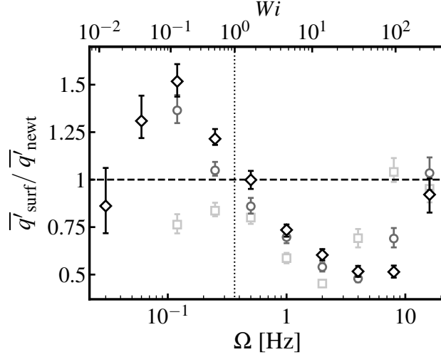
FIG. 6. Ratio of spatially averaged velocity fluctuation RMS \overline{q'} between the surfactant and Newtonian cases. Vertical dashed line represents the rotation rate for which Wi \approx 1 considering a relaxation time of \tau_s = 0.1 s. Darker markers indicate higher solution concentration, with the squares denoting 33 ppm, circles denoting 50 ppm and diamonds denoting 100 ppm solution.
