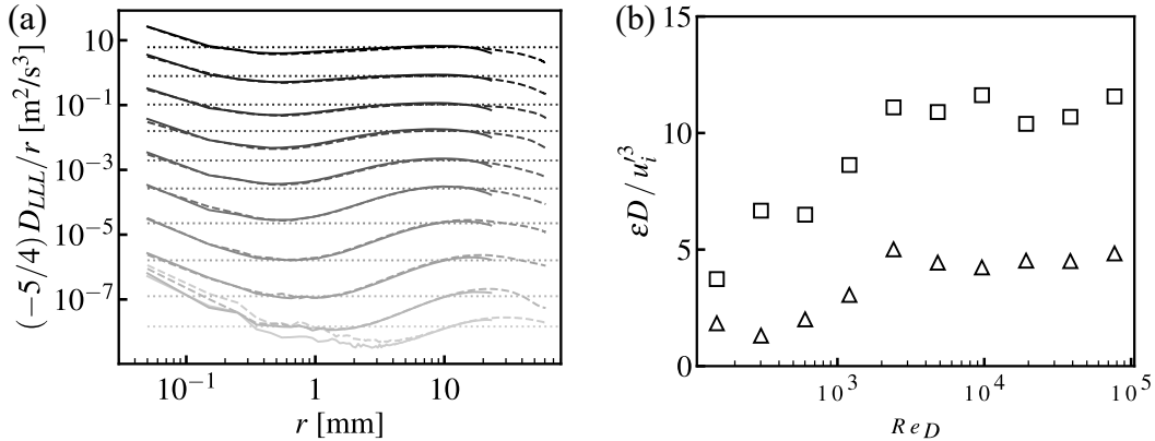
FIG. 4. (a) Compensated longitudinal third-order structure function, -5D_{LLL}^{(i)}(r)/(4r) , versus separation r for the Newtonian cases. Solid and dashed curves correspond to the two measured directions; darker curves indicate higher blade rotation rates. Dotted horizontal lines show the dissipation estimates obtained by averaging over 3 \leq r \leq 20 mm. (b) Dimensionless dissipation estimates, \varepsilon_i D / \overline{u_i'}^3 , versus blade Reynolds number Re_D . Triangles denote the horizontal direction ( i = x ); squares denote the vertical direction ( i = y ).
