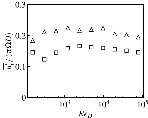
FIG. 3. Spatially averaged root-mean-square velocity fluctuations in the bulk, normalized by \pi \Omega D , versus the blade Reynolds number Re_D . Triangles denote the horizontal component ( u ); squares denote the vertical component ( v ).
