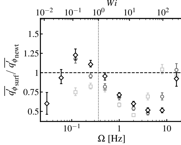
FIG. 11. Ratio of spatially averaged, phase-corrected velocity fluctuation RMS \overline{q'_{\phi}} between the surfactant and Newtonian cases. Darker markers indicate higher solution concentration, with the squares denoting 33 ppm, circles denoting 50 ppm and diamonds denoting 100 ppm solution.
