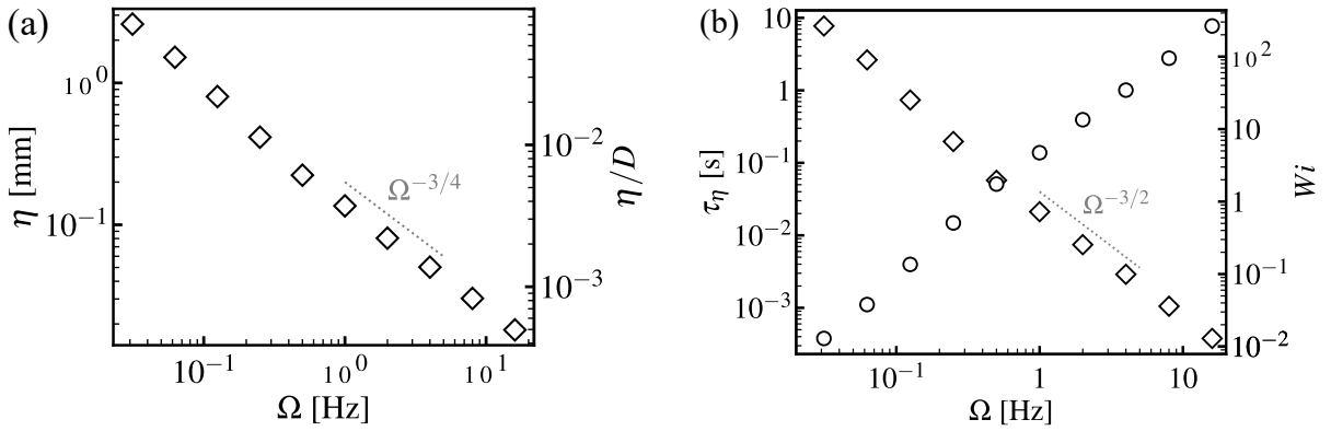
FIG. 5. (a) Kolmogorov length scale \eta versus blade rotation rate \Omega ; diamonds denote the estimates and the dotted line indicates the \Omega^{-3/4} scaling. (b) Kolmogorov time scale \tau_\eta (diamonds, left axis) and estimated Weissenberg number Wi (circles, right axis) versus \Omega . The dotted line indicates the \Omega^{-3/2} scaling; Wi is calculated using \tau_s = 0.1 s.
