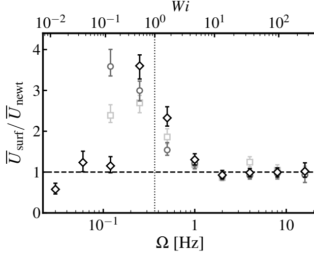
FIG. 7. Ratio of the signed, spatially averaged horizontal mean flow component \bar{U} between the surfactant and Newtonian cases. Vertical dashed line represents Wi \approx 1 . Darker markers indicate higher solution concentration, with the squares denoting 33 ppm, circles denoting 50 ppm and diamonds denoting 100 ppm solution.
