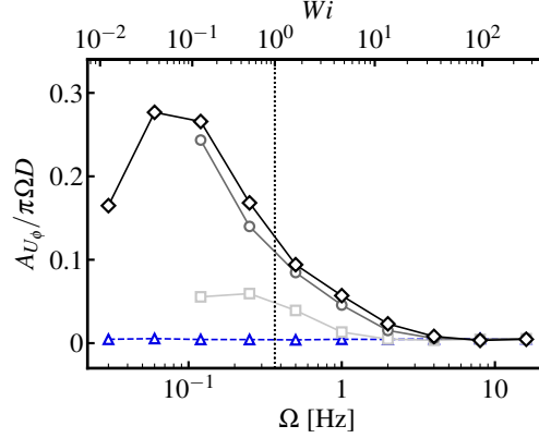
FIG. 9. Oscillation amplitude of the spatially averaged, phase-locked horizontal component of the mean flow, defined as half the peak-to-peak range and normalized by blade tip speed, A_{U_\phi}/(\pi\Omega D) , as a function of rotation rate. Grayscale curves denote surfactant solutions with darker markers indicating higher solution concentration. Squares denote 33 ppm, circles denote 50 ppm and diamonds denote 100 ppm solution. The blue line with triangle markers denotes Newtonian flow.
