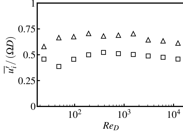
FIG. 3. Spatially averaged root-mean-square velocity fluctuations in the bulk, normalized by \Omega D , versus the blade Reynolds number Re_D . Triangles denote the horizontal component ( u ); squares denote the vertical component ( v ).
