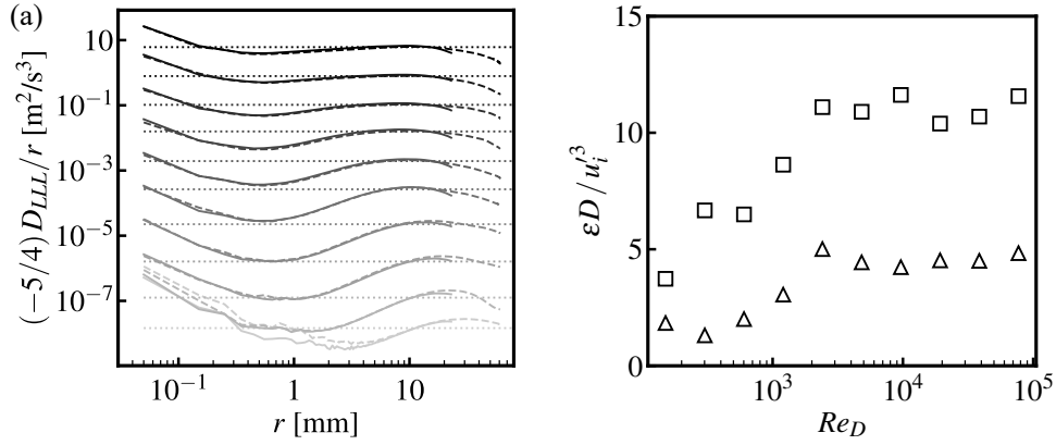
FIG. 4. (a) Compensated longitudinal third-order structure function, -5D_{LLL}^{(i)}(r)/(4r) , versus separation r for the Newtonian cases. Solid and dashed curves correspond to the two measured directions; darker curves indicate higher blade rotation rates. Dotted horizontal lines show the dissipation estimates obtained by averaging over 3 \leq r \leq 20 mm. (b) Dimensionless dissipation estimates, \varepsilon_i D / \overline{u'_i}^3 , versus blade Reynolds number Re_D . Triangles denote the horizontal direction ( i = x ); squares denote the vertical direction ( i = y ).
