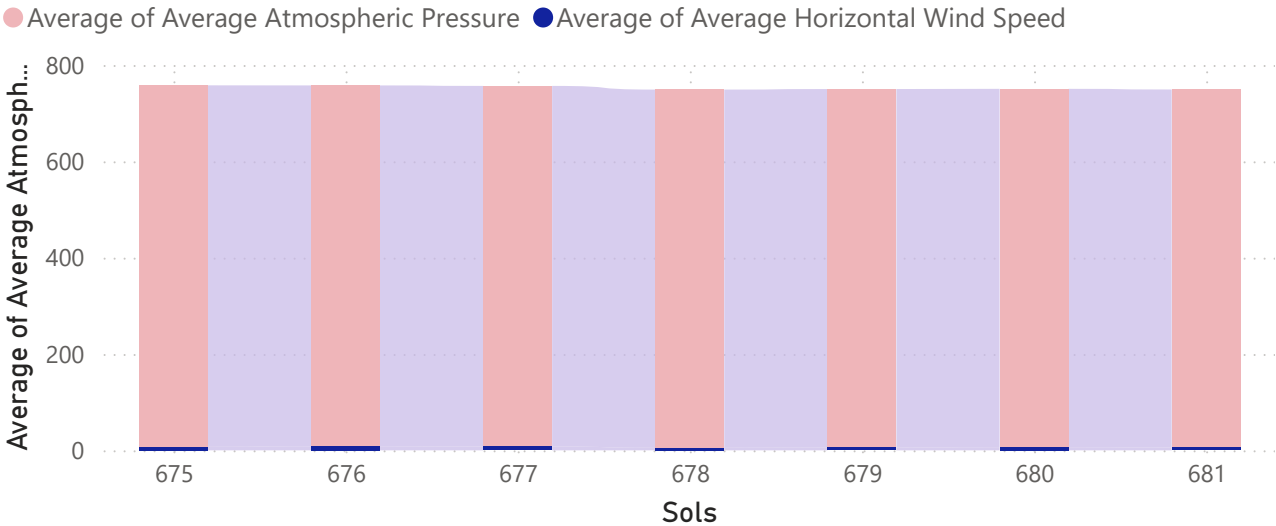
Average of Atmospheric Pressure and Average of Horizontal Wind Speed by Sols
