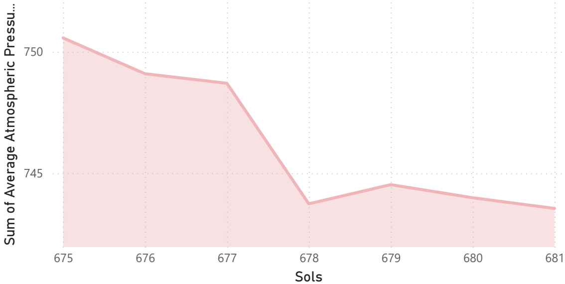
Sum of Average Atmospheric Pressure by Sols
