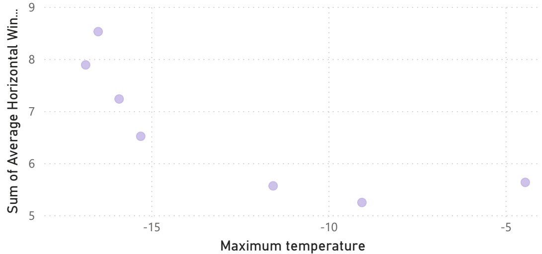
Sum of Average Horizontal Wind Speed by Maximum temperature
