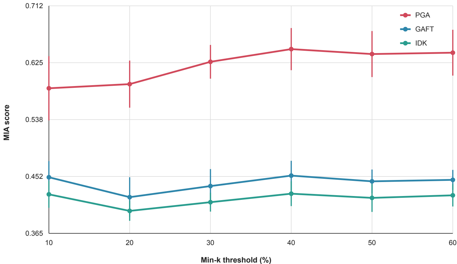
MIA Sensitivity Across Min-k Thresholds
