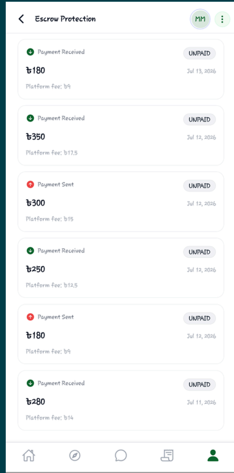
Escrow Payment
