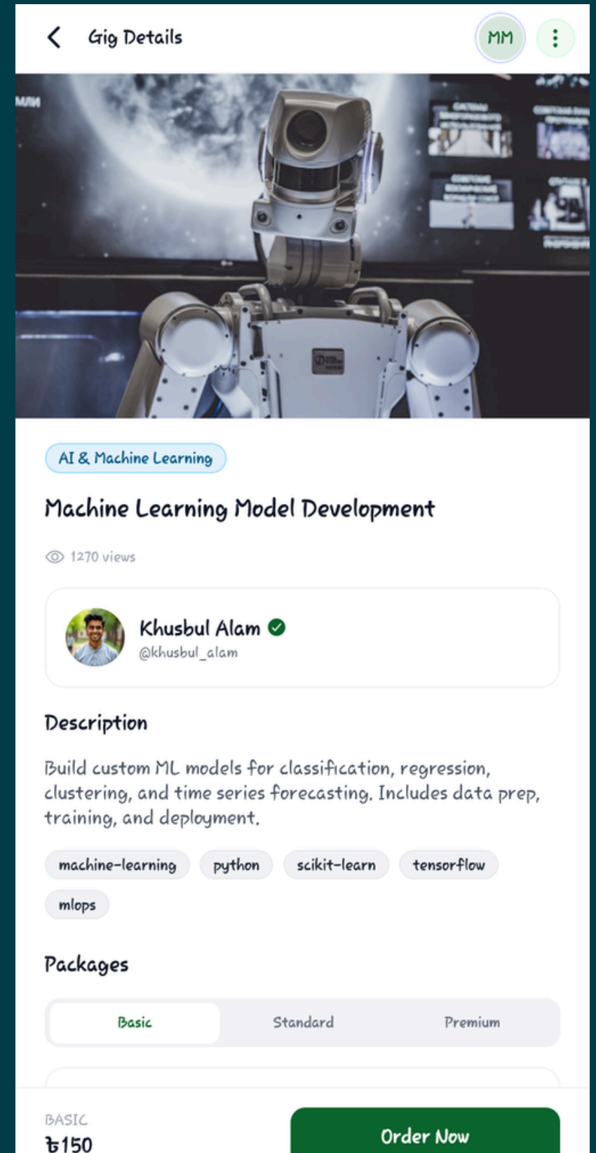
Job Description
