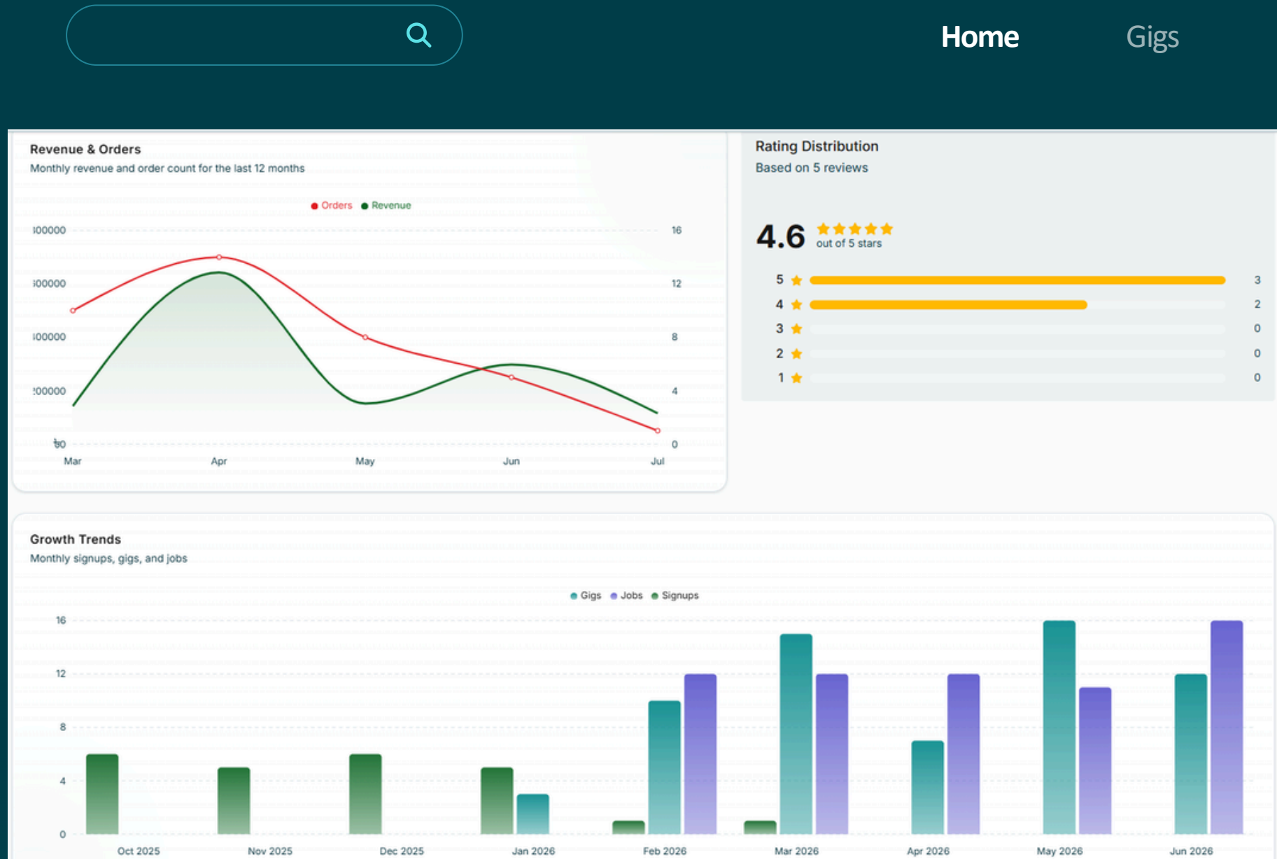
Admin Dashboard
