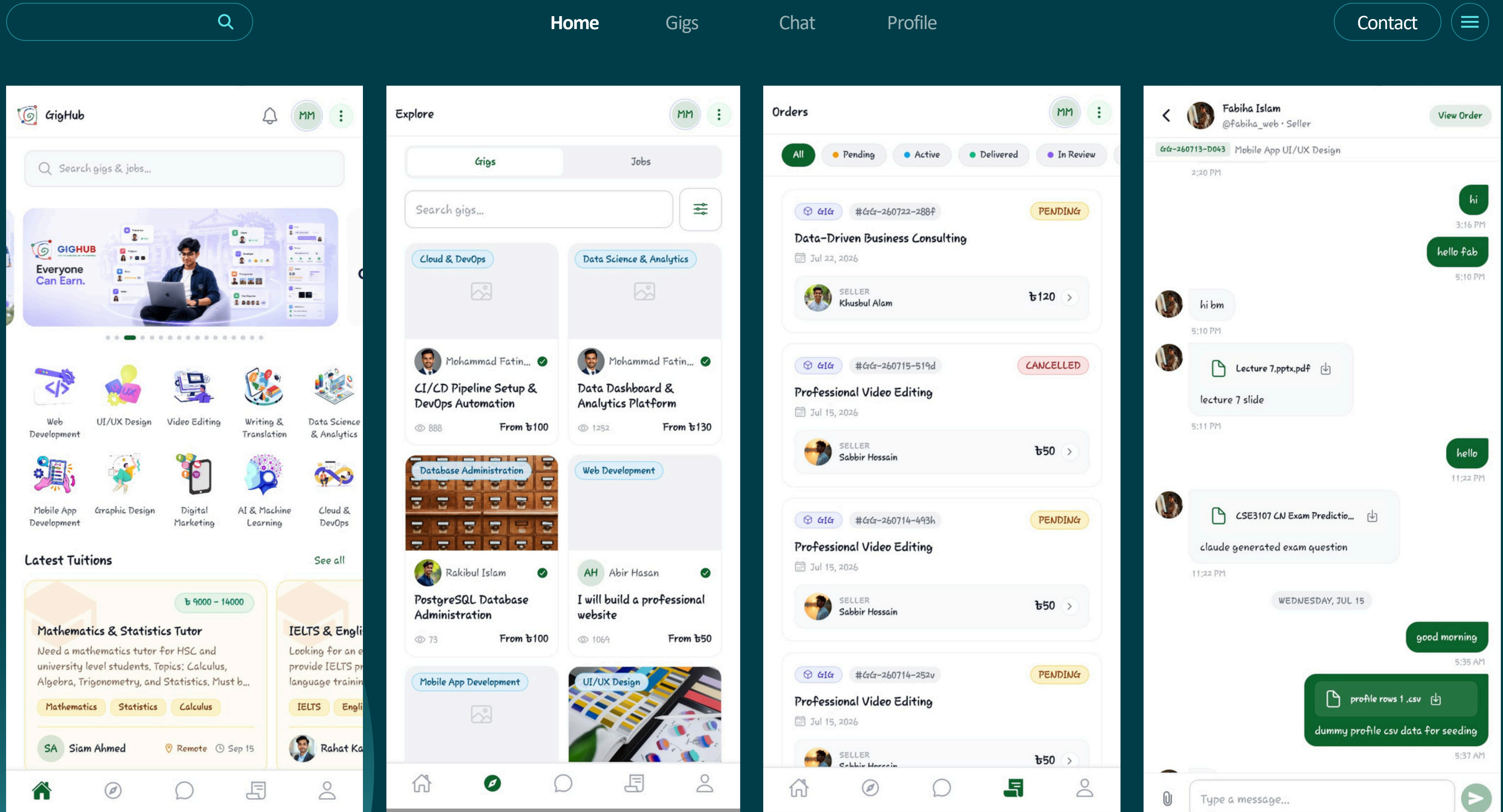
Homepage
