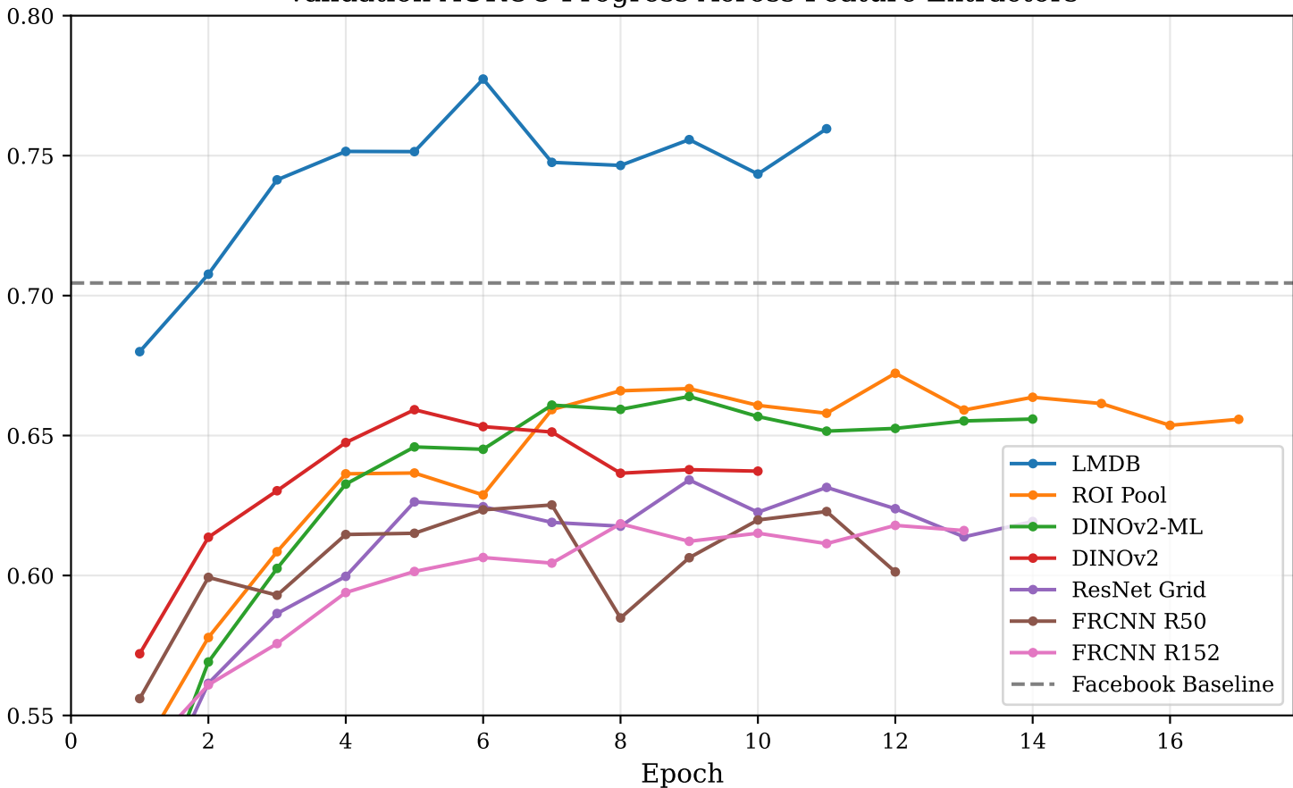
Validation AUROC Progress Across Feature Extractors
