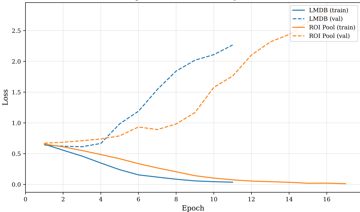
Training and Validation Loss (Top 2 Models)
