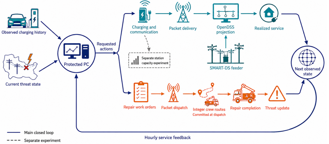
Fig. 1. Executable PC closed loop. Protected PC denotes PC with reference protection. Observed charging history supplies the shared forecast, and the controller receives the current scenario threat state. EAGLE-I observations inform transition calibration and the repair duration prior. Requested service actions pass through packet delivery and SMART-DS/OpenDSS projection. Repair work orders pass through packet dispatch, integer routing, and recorded completion events. Routes are committed at dispatch, while service allocations are updated hourly. Realized service and threat updates form the next observed state. The dashed path denotes the separate station capacity experiment and is not part of the primary 4,096-scenario loop. The conceptual illustration was generated and edited with OpenAI image tools, https://openai.com/ .
