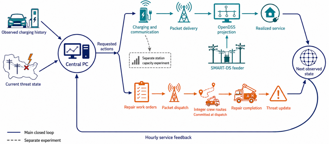
Fig. 1. Executable PC closed loop. Observed charging history supplies the shared forecast, and the controller receives the current scenario threat state. EAGLE-I observations inform transition calibration and the repair duration prior. Requested service actions pass through packet delivery and SMART-DS/OpenDSS projection. Repair work orders pass through packet dispatch, integer routing, and recorded completion events. Routes are committed at dispatch, while service allocations are updated hourly. Realized service and threat updates form the next observed state. The dashed path denotes the separate station capacity experiment and is not part of the primary 4,096-scenario loop. The conceptual illustration was generated and edited with OpenAI image tools, https://openai.com/ .
