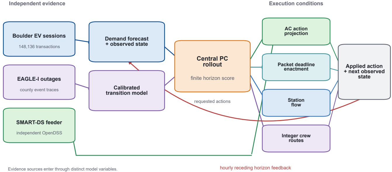
Fig. 1. Executable PC closed loop. Boulder charging sessions supply measured demand and forecasts. EAGLE-I supplies county level outage calibration. SMART-DS independently constrains feeder action. PC rollout issues requested actions, while service and threat states change only after distribution system projection, packet deadline enactment, station flow, and integer crew routing. The next observation restarts the hourly horizon. The three public sources serve distinct model roles.
