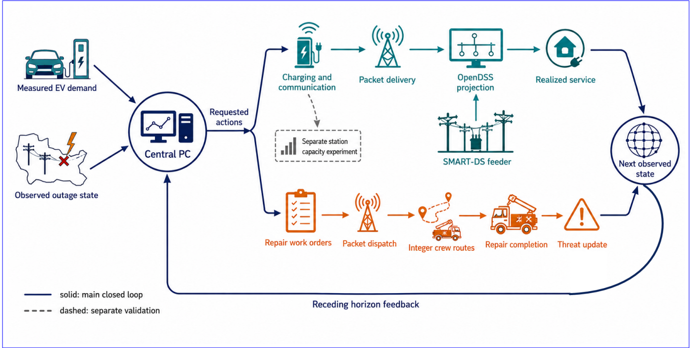
Fig. 1. Executable PC closed loop. Boulder charging demand and EAGLE-I outage states inform central PC. Requested service actions pass through packet delivery and SMART-DS/OpenDSS projection. Repair work orders pass through packet dispatch, integer routing, and recorded completion events. Realized service and threat updates form the next observed state. The dashed path denotes the separate station capacity experiment and is not part of the primary 4,096-scenario loop.
