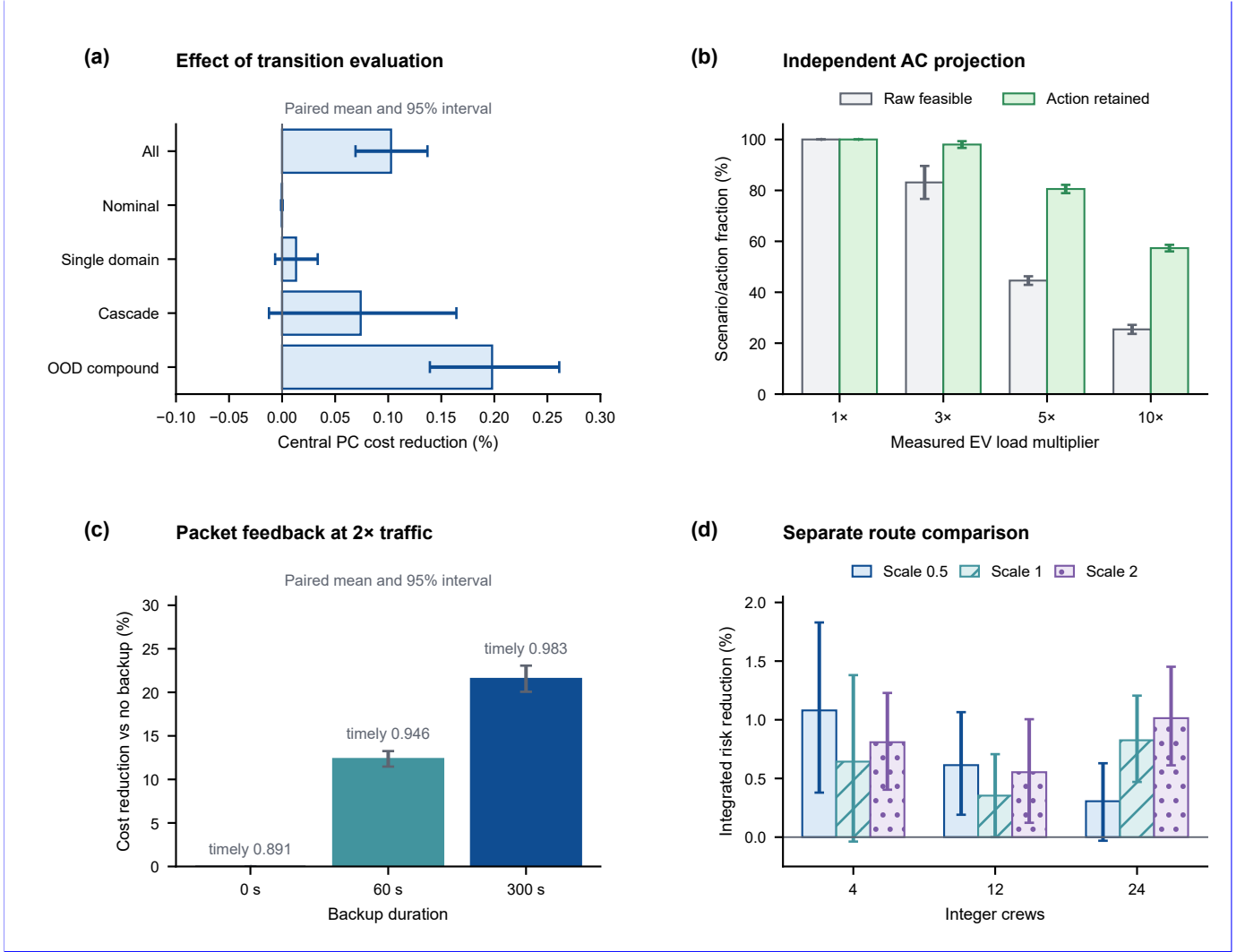
Fig. 2. Decision and execution evidence. Panel (a) reports the central PC cost reduction relative to the forecast matched baseline. Filled intervals show paired means and bootstrap confidence limits for each threat class and for all scenarios. Panel (b) reports raw distribution system feasibility and the fraction of requested EV action retained after projection, with normal approximation intervals across 20 mappings of 24 hours each. Panel (c) reports the cost reduction from backup power under increased packet traffic, with the mean fraction of actions delivered on time printed above each bar. Panel (d) reports the separate integrated risk comparison when executable routes are evaluated before selection. Panels (a), (c), and (d) show paired bootstrap 95% intervals, using 4,096 pairs overall and 1,024 per class in (a), 1,024 in (c), and 128 per crew and service condition in (d). Paired t and Wilcoxon tests with their stated Holm families are reported in the tables. Percentage intervals divide the cost or risk difference interval by the observed reference mean.
