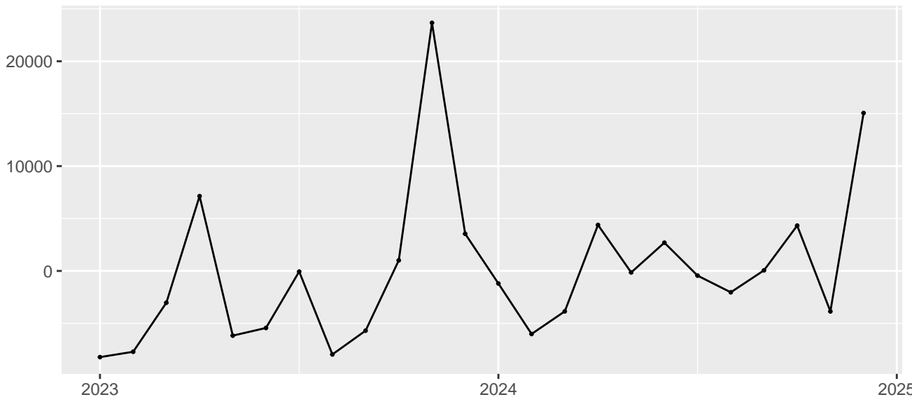
Residuals from ARIMA(0,0,0) with non-zero mean
