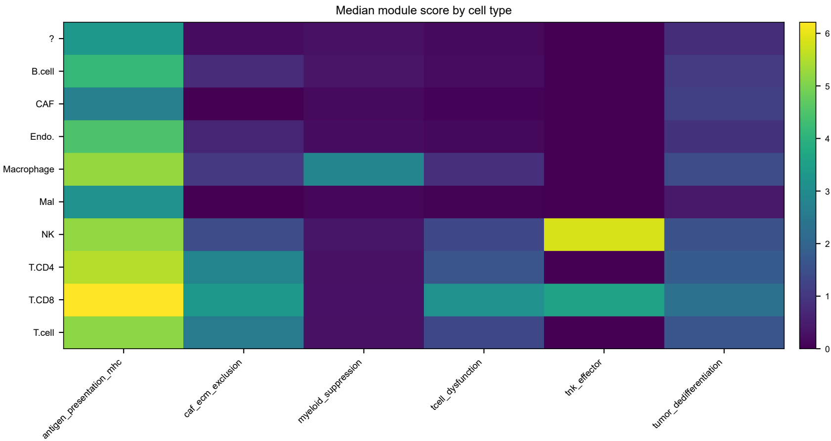
Supplementary Fig. 9 | Single-cell and ecological mechanism
