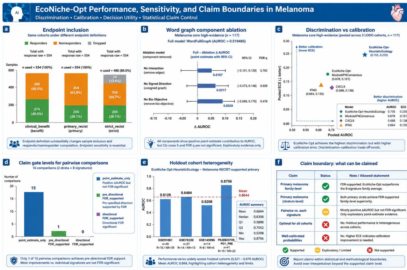
Figure 4 | Endpoint sensitivity and ablation analyses strengthen the evidence hierarchy.
