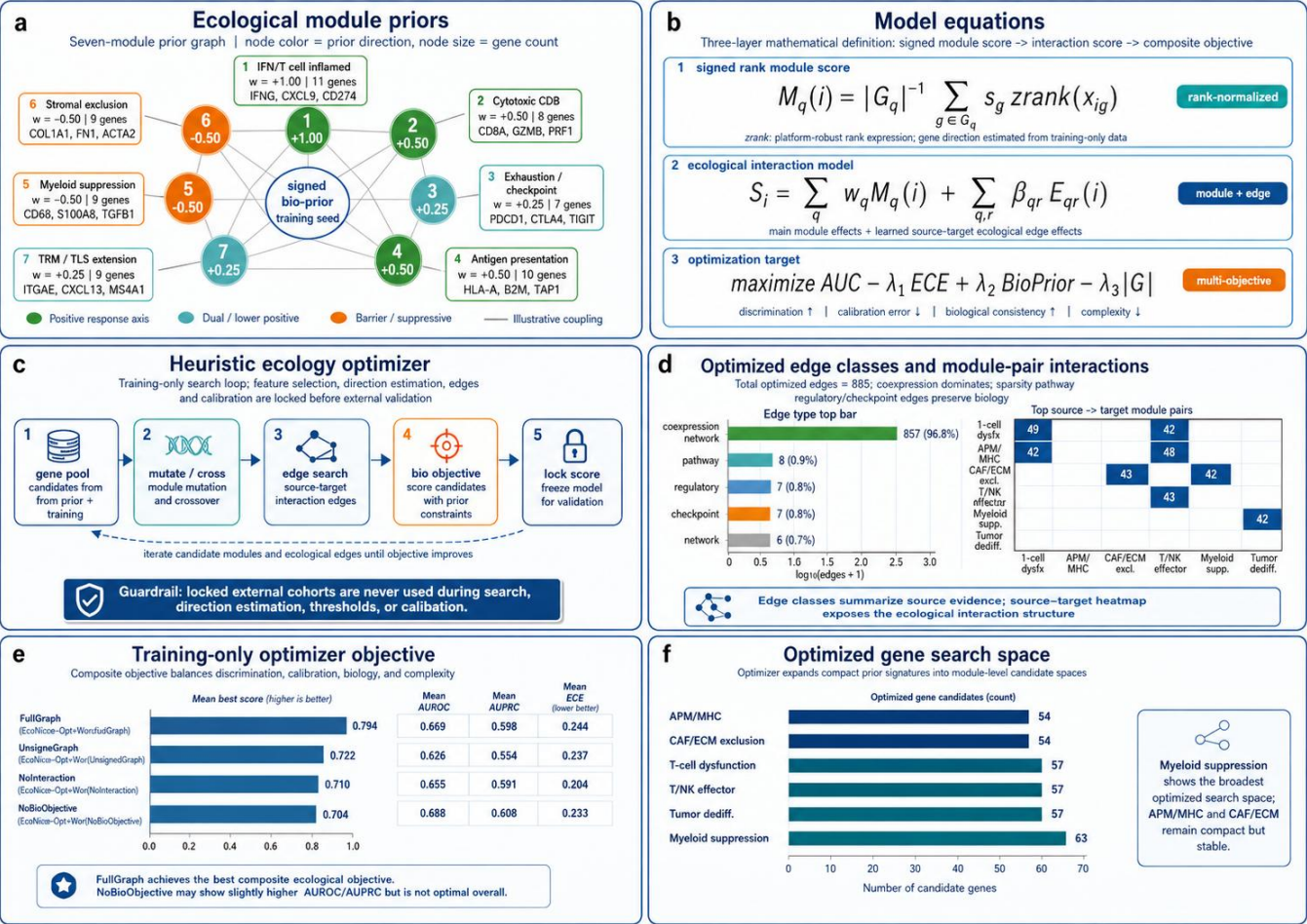
Figure 2 | EcoNiche-Opt converts immune states into a coupled ecological score.
