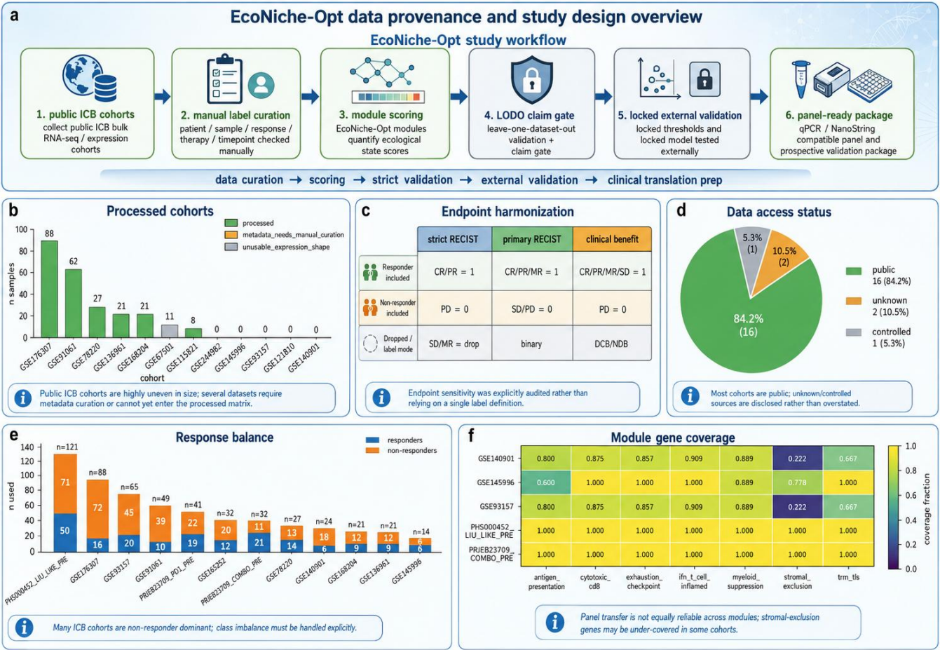
Figure 1 | Building an auditable multicohort ICB response benchmark.
