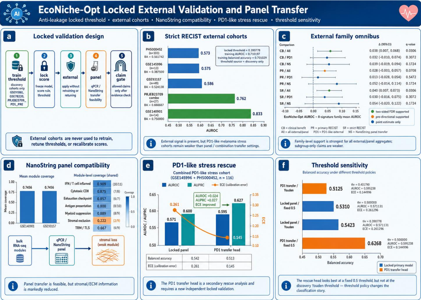
Figure 5 | Locked external and panel-transfer scoring evaluates portability without refitting.
