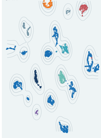
target-cohort geometry
