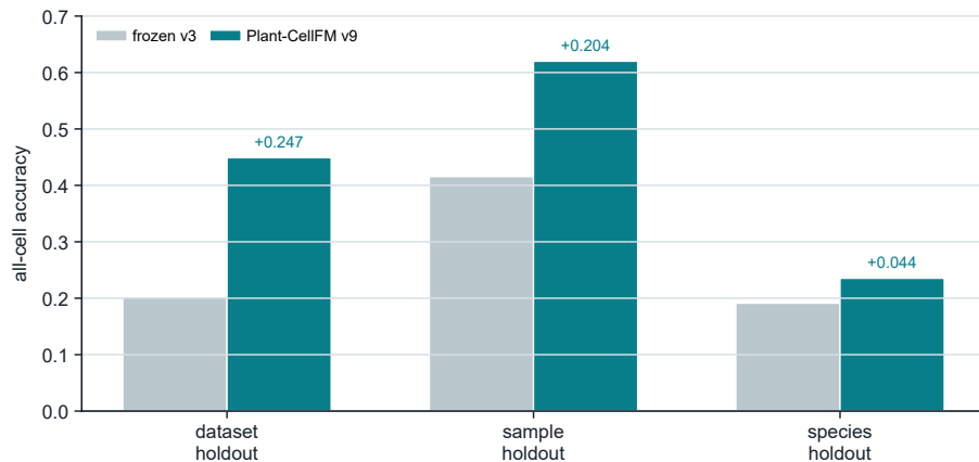
Frozen checkpoint gains under matched grouped splits
