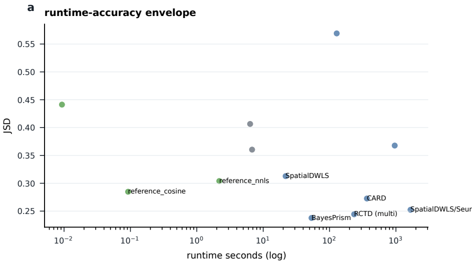
Fig. 15 | Compute and scalability Runtime-accuracy and memory profiles provide methods-oriented reproducibility context.
