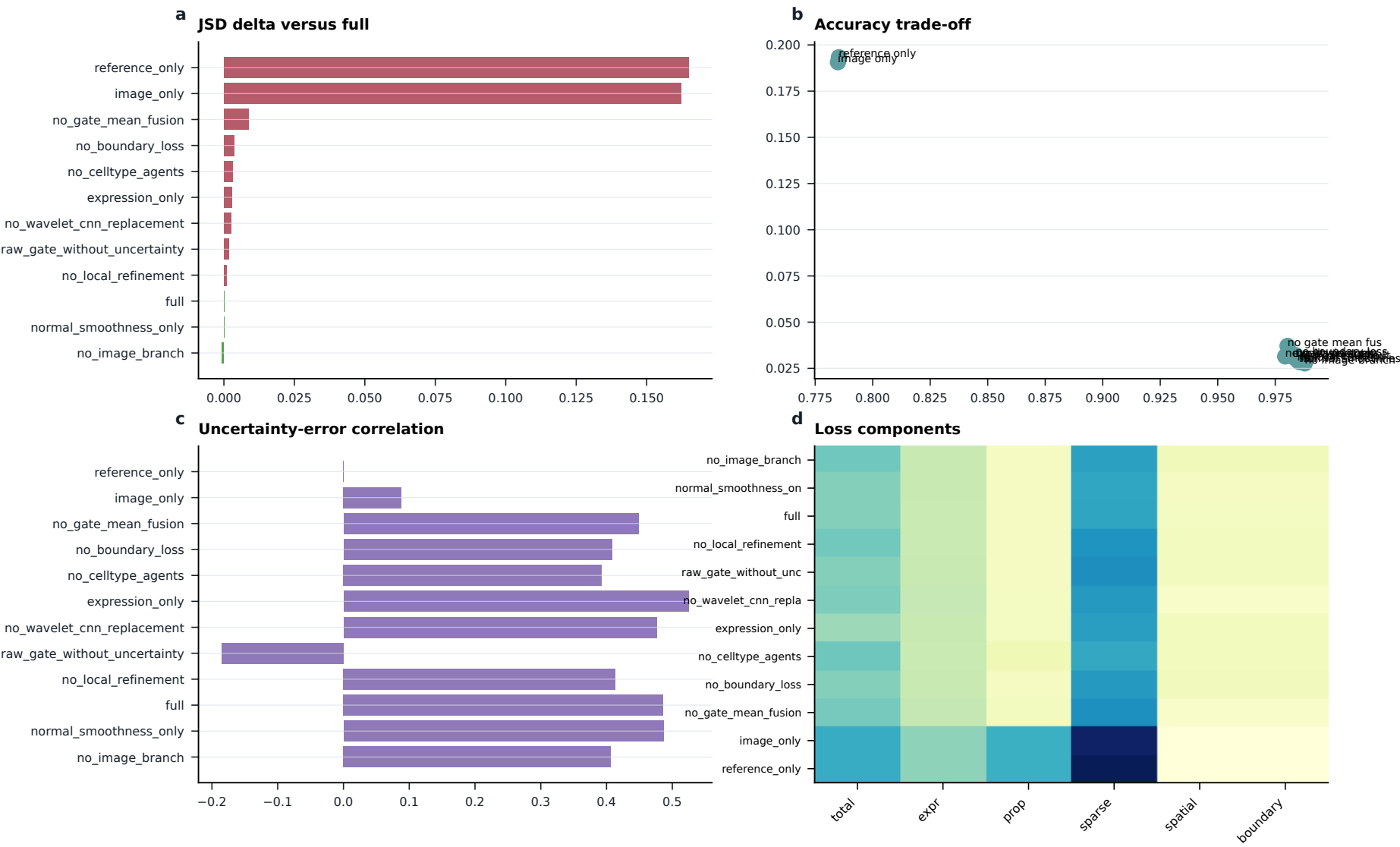
Fig. 6 | Ablation mechanism wall Module and modality removals quantify necessity across accuracy, uncertainty and boundary-aware objectives.
