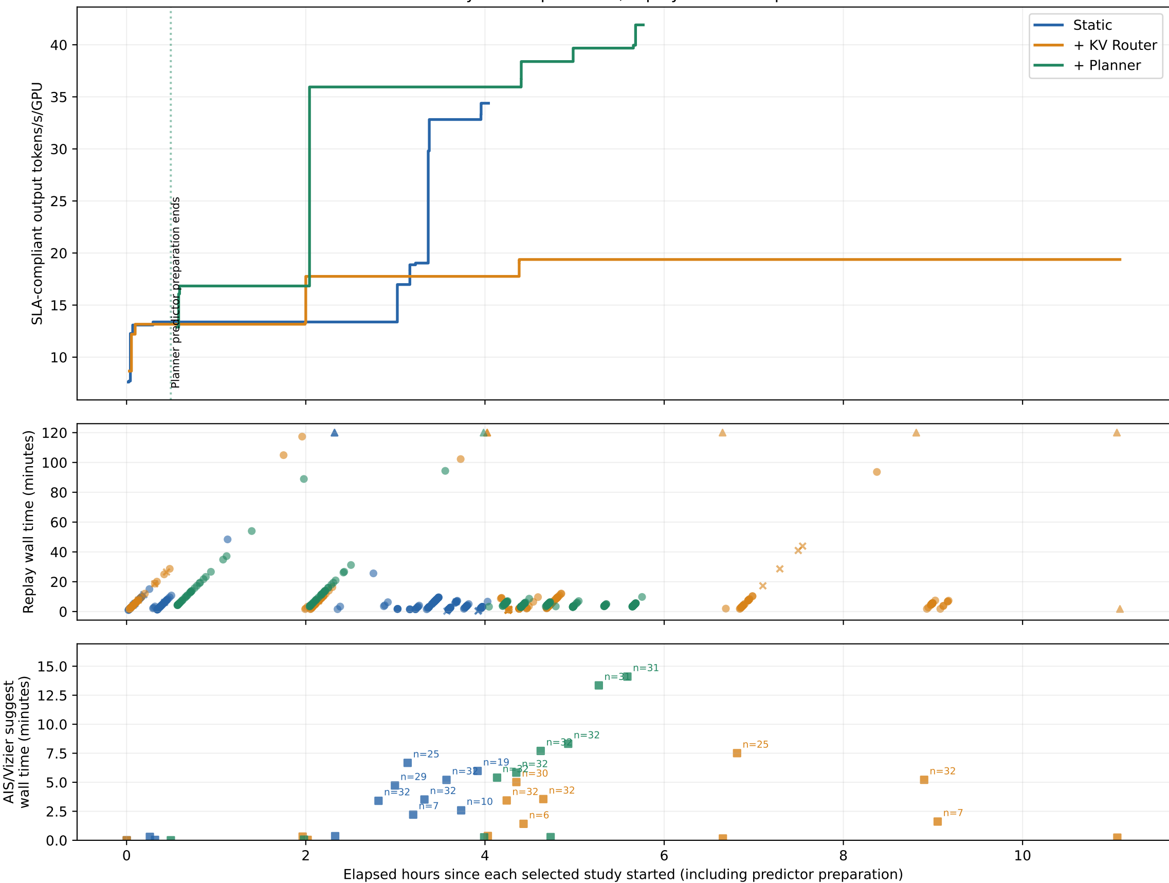
RAGPulse day 5: accepted best, replay time and optimizer time
