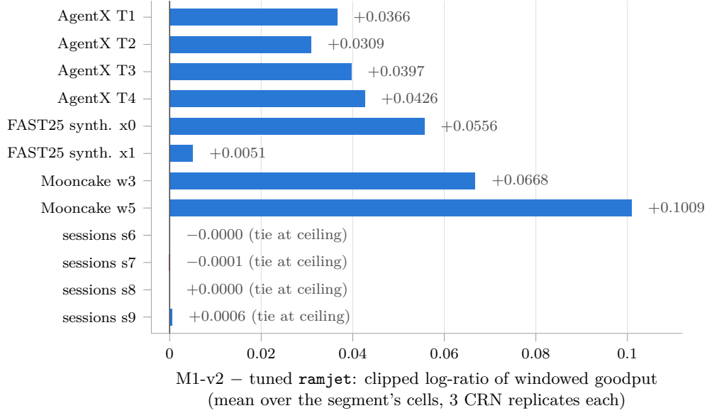
Figure 7: The headline per test segment, labeled by family and the segment names of Table 9. The four session segments tie at ceiling; every other segment favors M1-v2.
