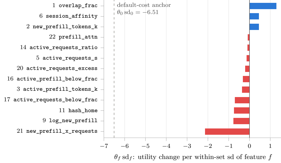
Figure 10: M1-v2’s nonzero coefficients, standardized, labeled with the feature index f and name of Table 12. Positive attracts a worker, negative repels it; the default-cost anchor is at -6.51 .
