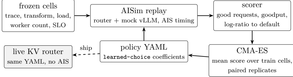
Figure 1: The training loop. A policy is a YAML file read by the router’s builtin policy catalog, so each CMA-ES candidate costs a new YAML and a set of replays, with no rebuild. Every candidate is scored on the same workload replicates, and its score is the clipped log-ratio of its windowed goodput to the default router’s. AIS times the simulated engines and so shapes the score; the headline policy never reads it.
