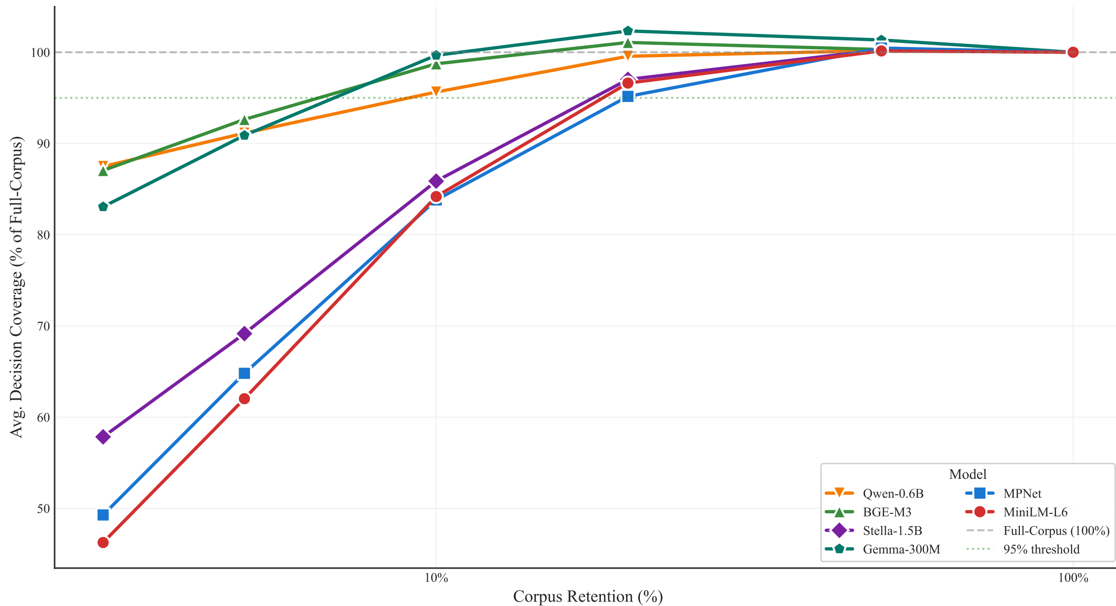
Normalized Avg. Decision Coverage: Degradation from Filtering (Budget=1000)
