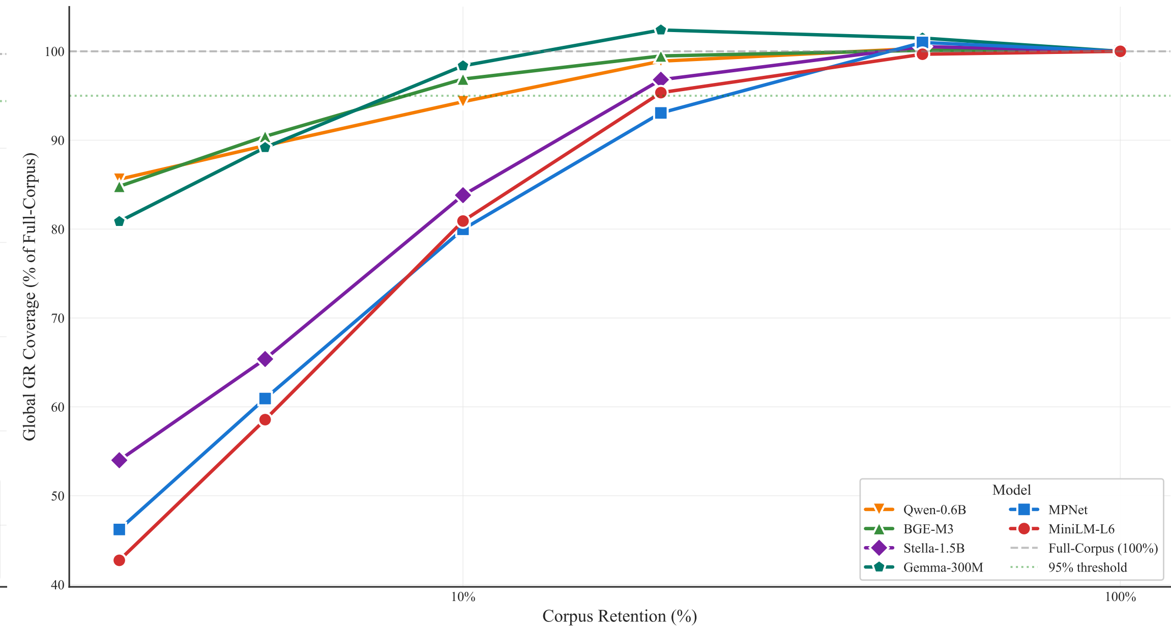
Normalized Global GR Coverage: Degradation from Filtering (Budget=1000)
