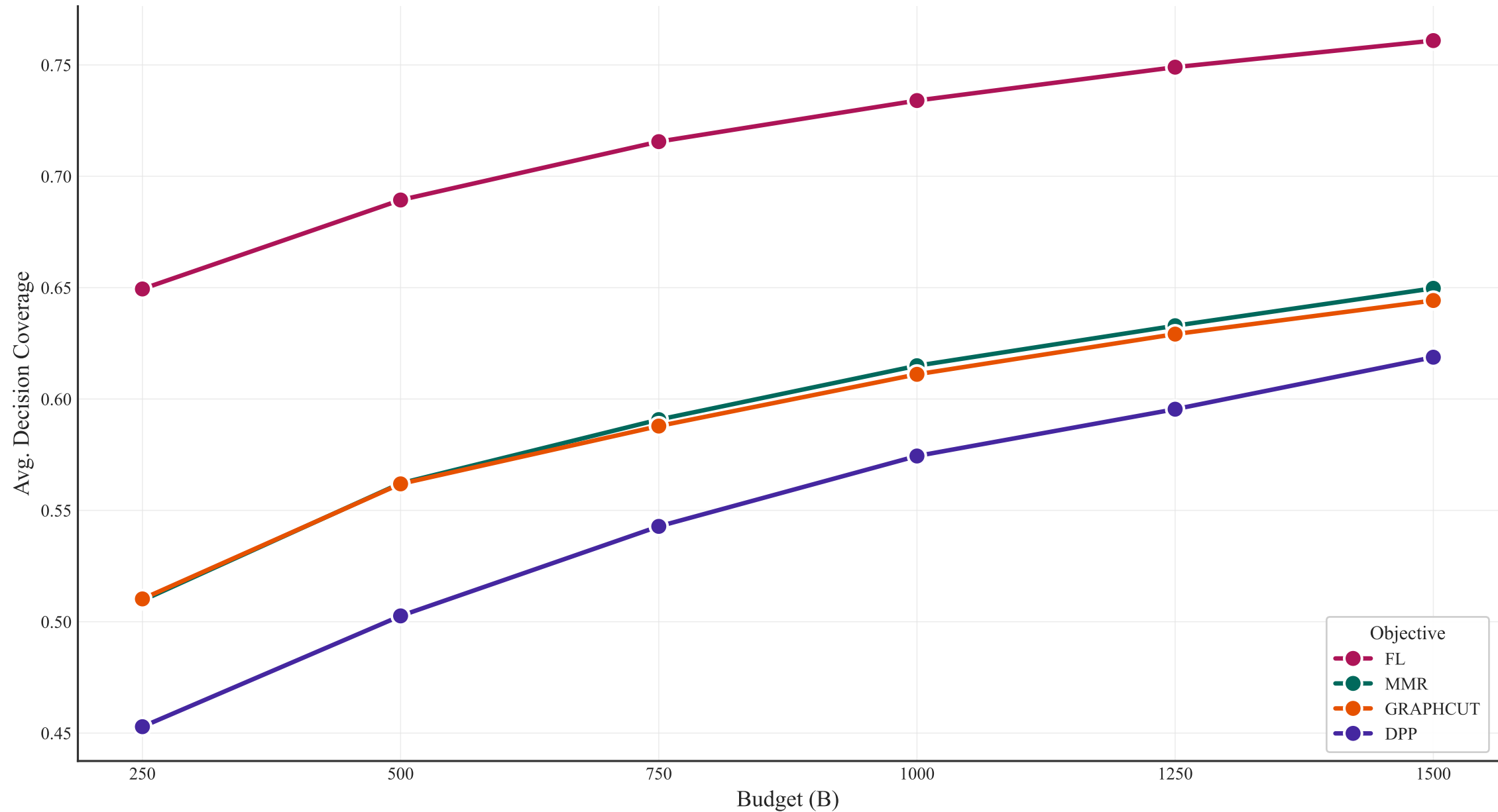
Budget Scaling by Objective: Avg. Decision Coverage (K-Means)
