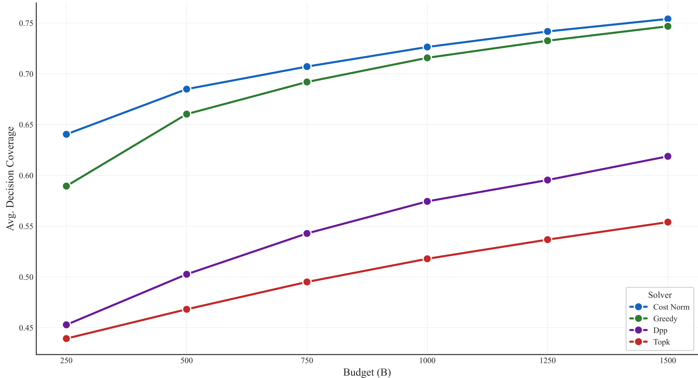
Budget Scaling by Solver: Avg. Decision Coverage (K-Means)
